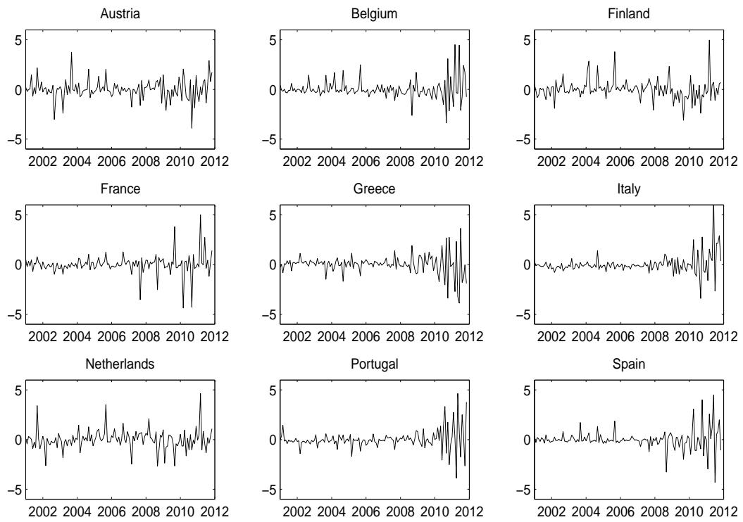
Figure 4: Standardized residuals from the panel regression
