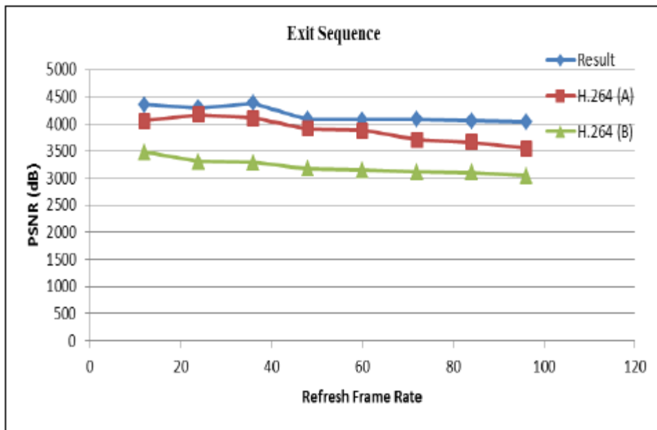
10. Performance of sequence Exit compared with two H.264 schemes
