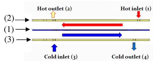
Figure 4-Flow scheme inside the HE
