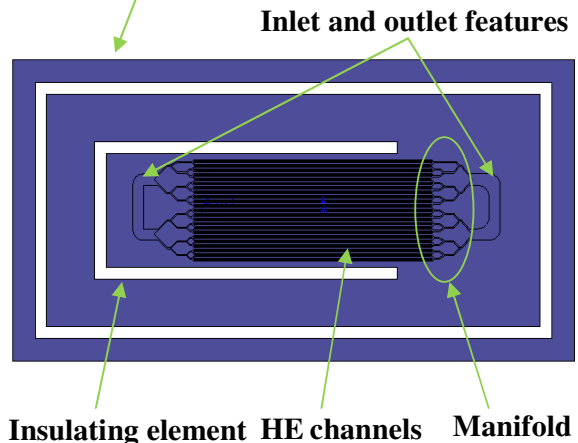
Figure 5-Silicon layer design
