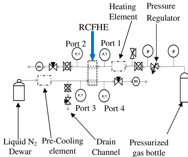
Figure 2a -scheme of the experimental test setup
