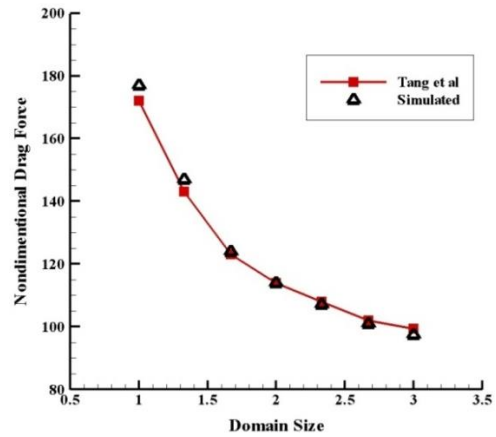
Fig. 6. Comparison of drag forces obtained from present simulation and reference [5]
