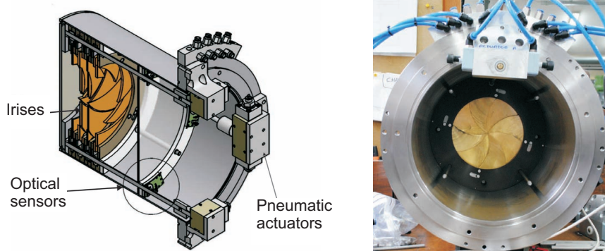
Figure 10. Left panel: schematic of the MICE diffuser showing the irises. Right panel: one of the brass irises being tested.
