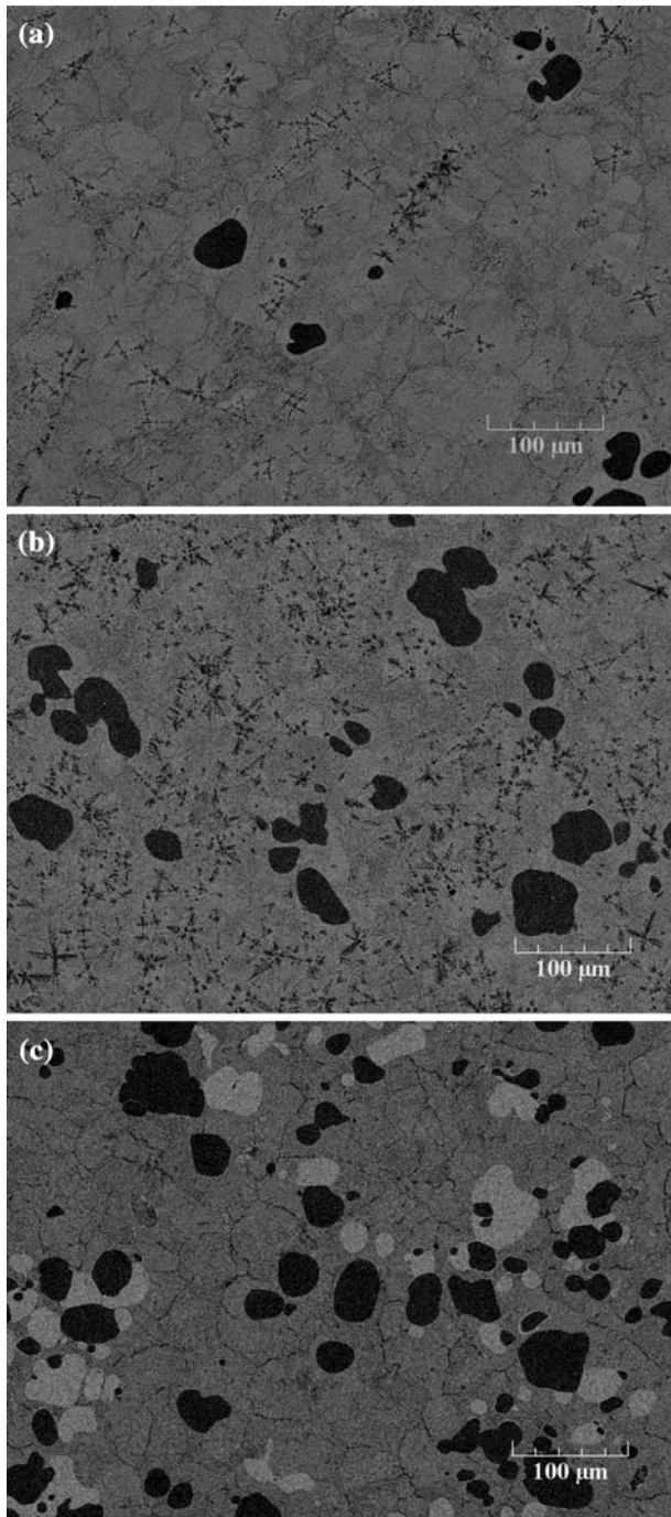
Fig. 10—Backscattered SEM micrographs showing water-quenched microstructures of Zn-6.3 wt pct Al alloy produced under shearing at 4082 \text{ s}^{-1} and cooling from 395 \text{ °C} at 1 \text{ °C/min} to different temperatures: (a) 391.2 \text{ °C} , (b) 389.4 \text{ °C} , and (c) 380.5 \text{ °C} (white particles = Zn phase, and black particles = Al phase).
