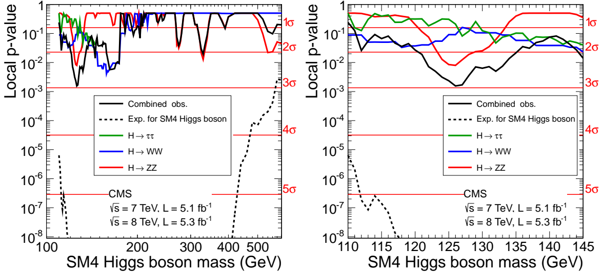
Figure 4: The observed local p -value p_0 as a function of the SM4 Higgs boson mass in the range 110–600 GeV (left) and 110–145 GeV (right). The dashed line shows the expected local p -values should an SM4 Higgs boson with a mass m_H exist. The expected p -value is obtained with nuisance parameters constrained by the data, giving it some dependence on the observed data, and hence the small modulations on top of the overall smooth trend as a function of m_H .
