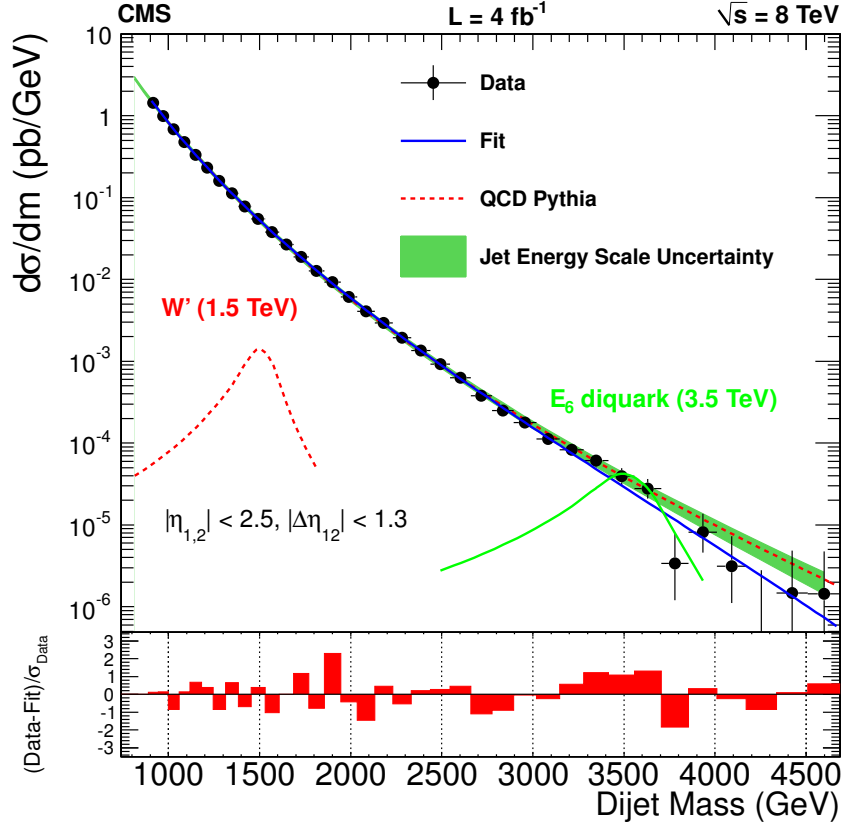
Figure 1: The dijet mass spectrum from wide jets (points) compared with a smooth fitted curve (solid line) and with the predicted QCD background [28] (dashed line). The QCD background curve has been normalized to the data (see text) and a linear smoothing between the bins has been applied. The vertical bars on the data points represent the statistical uncertainty, the horizontal bars indicate the bin widths. The shaded band shows the contribution from the systematic uncertainty in the jet energy scale. Also shown are the predictions for a W' boson with a mass of 1.5 TeV, and an E_6 diquark with a mass of 3.5 TeV, obtained fitting the expected distribution to a Crystal ball [29] function and normalizing the area to the predicted cross section. The bottom part of the plot displays the bin-by-bin residuals (data minus the integral over a bin of the smooth function fitted to the data) divided by the statistical uncertainty in the data.
