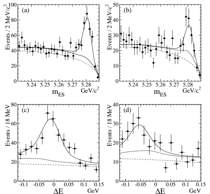
FIG. 1: Distributions of m_{ES} and \Delta E for samples enhanced in \rho\pi signal (a,c) and \rho K signal (b,d). The solid curve represents a projection of the maximum likelihood fit result. The dashed curve represents the contribution from continuum events, and the dotted line indicates the combined contributions from continuum events and B -related backgrounds.
