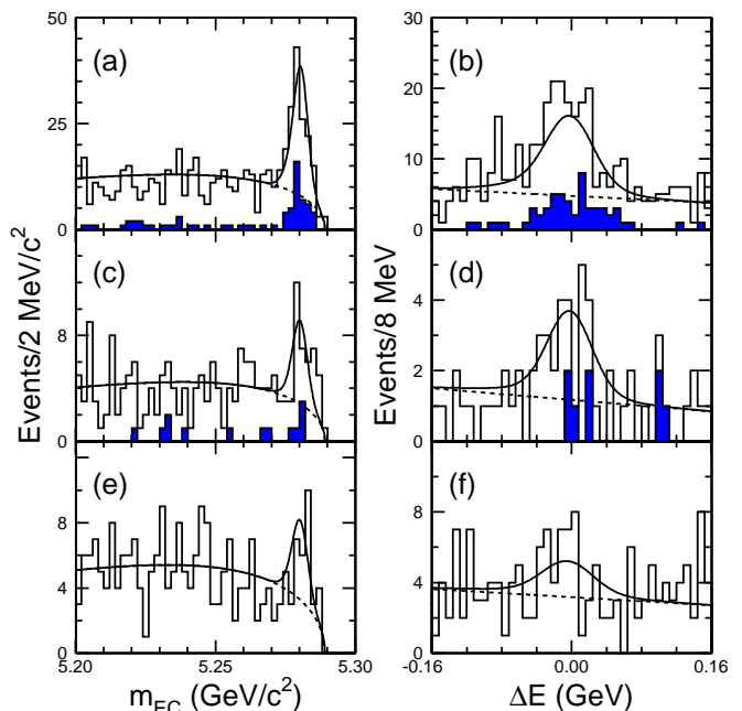
FIG. 2: B candidate m_{EC} and \Delta E for B^+ \rightarrow \eta'K^+ (a, b), B^0 \rightarrow \eta'K^0 (c, d), and B^+ \rightarrow \omega\pi^+ (e, f). Histograms represent data, with the \eta' \rightarrow \eta\pi\pi subset shaded, solid curves represent the full fit functions, and dashed curves the background functions.
