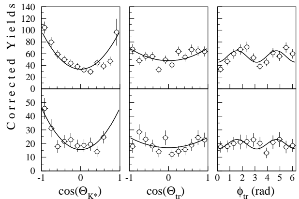
FIG. 2: The angular distributions for the channels with (top) and without (bottom) a \pi^0 for m_{\text{ES}} > 5.27 \text{ GeV}/c^2 . The data have been background-subtracted and acceptance-corrected. The curves correspond to the fit.
