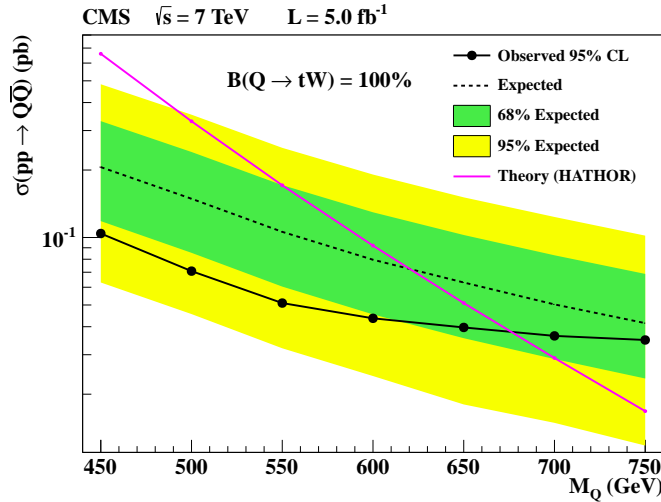
Figure 2: The observed (solid line with points) and the expected (dashed line) 95% CL upper limits on the Q\bar{Q} production cross section as a function of the heavy quark mass, M_Q , compared to the theoretical Q\bar{Q} cross section for the case of a down-type heavy quark decaying exclusively to tW .
