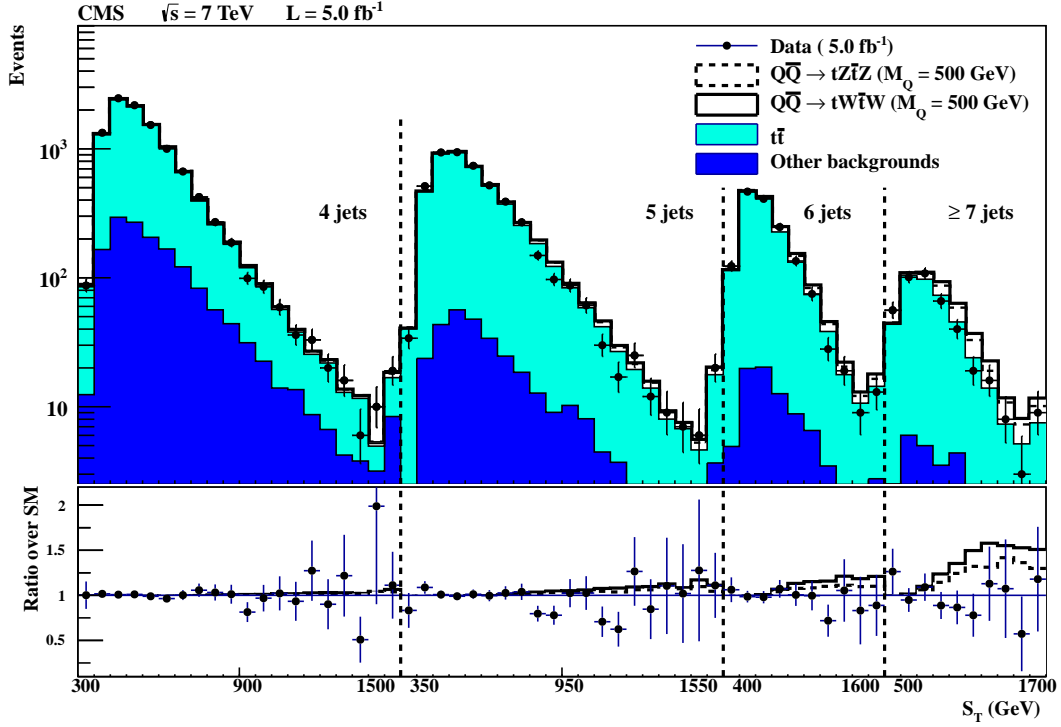
Figure 1: Distribution in S_T for different jet multiplicities after the maximum-likelihood fit to data. The last bin in each subfigure is the overflow bin. The bottom plot shows the ratios of data and SM plus signal over SM. Q \rightarrow tW and Q \rightarrow tZ distributions are shown for illustrative purposes for M_Q = 500 GeV.
