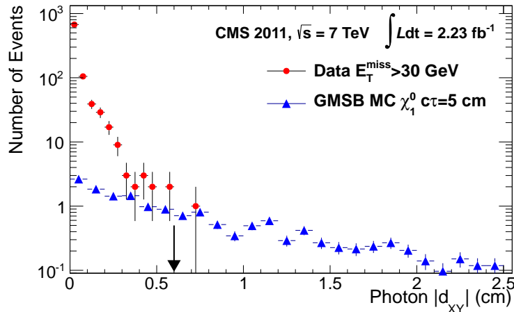
Figure 3: The |d_{XY}| distribution for data with E_T^{\text{miss}} > 30 GeV compared with signal simulation for c\tau = 5 cm normalized to the integrated luminosity of the data. The arrow indicates the |d_{XY}| requirement of the signal region.
