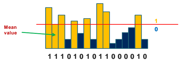
Fig. 8. A sample 16 bin histogram. The binary signature is extracted by thresholding at the mean bin frequency value.
