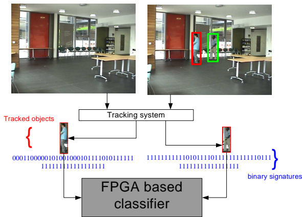
Fig. 9. Processing of objects for identification. The tracking system detects objects and constructs a bounding box. A binary signature is extracted from the colour histogram of each object, and fed to the bSOM for identification.
