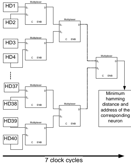
Fig. 4. Structure of the minimum Schema distance unit in the WTA unit.
