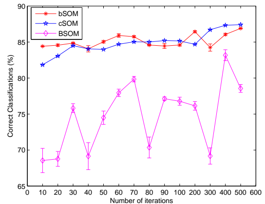
Fig. 11. Performance of the three different SOM implementations for 10, 20, 30, 40, 50, 60, 70, 80, 90, 100, 200, 300, 400 and 500 iterations using binary signatures extracted from the colour histogram for nine objects.
