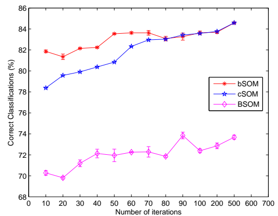
Fig. 6. Performance of the three different SOM implementations for different iteration counts. The average correct classification rate is illustrated with error bars.
