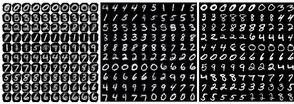
Fig. 7. Results of the three implementations using the [31] dataset. Left: original SOM (cSOM); middle: tri-state SOM (bSOM); right strict binary SOM (BSOM). In cSOM grey-levels are used to illustrate weight magnitude; in BSOM # is represented by mid-grey.
