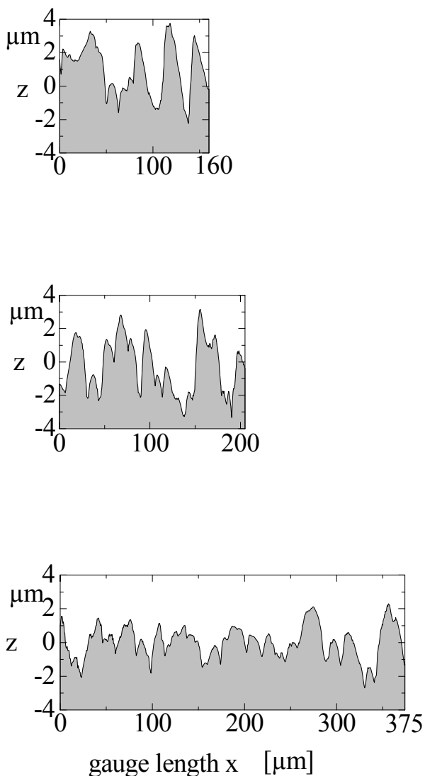
Figure 5: Representative profiles of the microchannels with different diameter ( D = 0.4 mm, top, D = 0.5 mm, middle, D = 0.8 mm, bottom). Enlargement: z/x = 6
