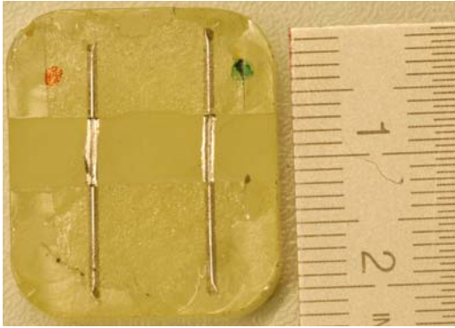
Figure 2: Microchannels of I.D. 0.4 mm embedded in epoxy after the milling and cutting process ready for the roughness measurements
