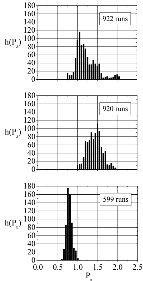
Figure 8: Probability distribution of the P_a values of the microchannels with different diameter 0.4 mm (top), 0.5 mm (middle), 0.8 mm (bottom)
