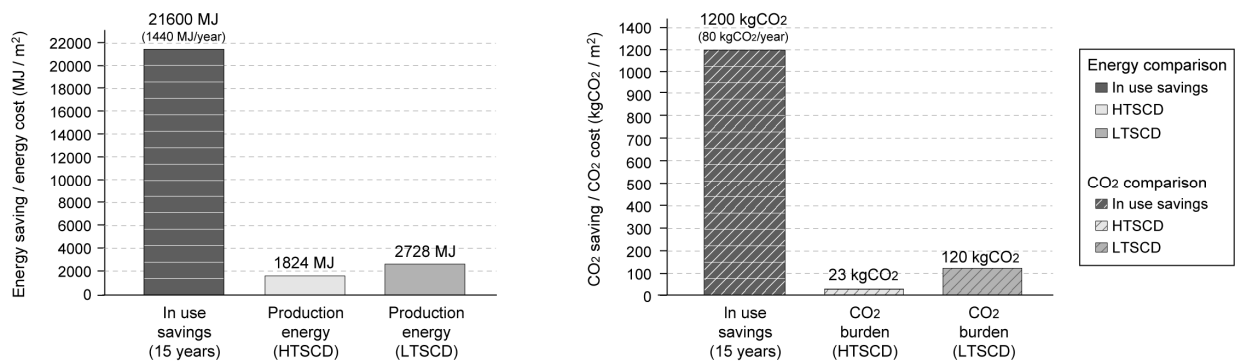
[Figure 9: Production costs of aerogel vs. in-use savings over product lifespan. Left graph compares production energy. Right graph compares CO 2 burden]
