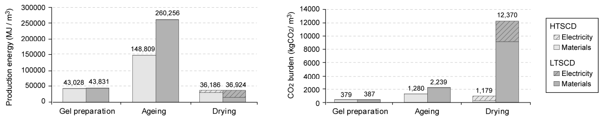
[Figure 8: Scaled production impact for making 1m 3 aerogel via HTSCD and LTSCD. Left graph compares production energy. Right graph compares CO 2 burden]
