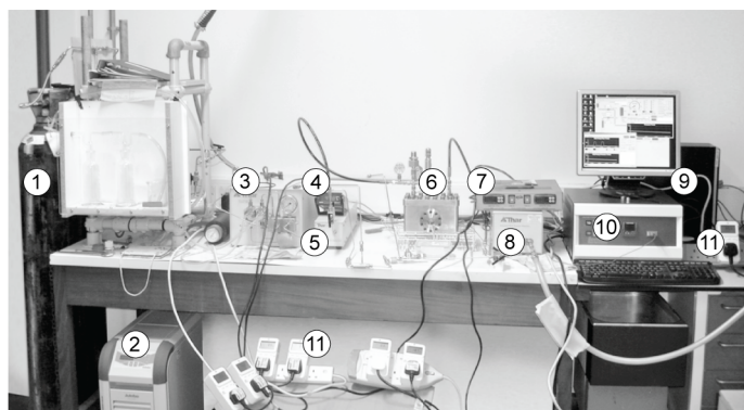
LTSCD: ④ Temperature sensor ⑧ Back pressure regulator ① CO 2 canister ⑤ Pipe heater ⑨ Computer & monitor ② Chiller ⑥ Autoclave ⑩ Autoclave heater controller ③ Pump ⑦ Pipe heater controller ⑪ Plug monitors
