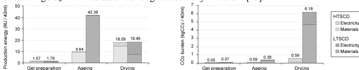
[Figure 7: Production impact associated with making 40ml aerogel via HTSCD and LTSCD. Left graph compares production energy. Right graph compares CO 2 burden]
