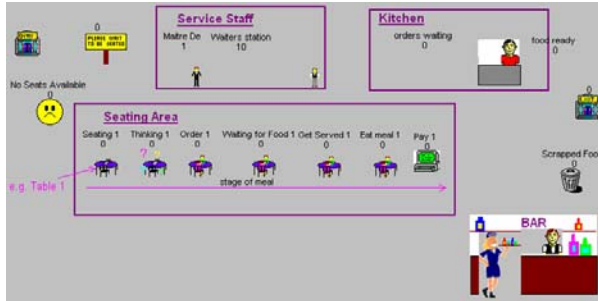
Figure 4. Simul8 Model
