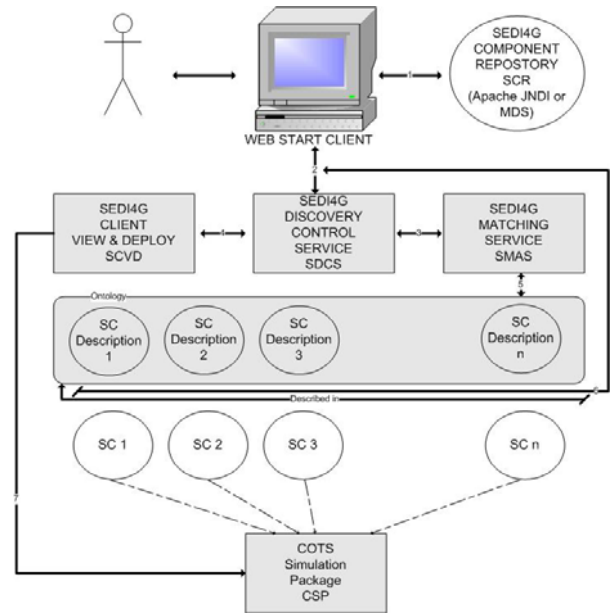
Figure 5. Discovery Architecture
