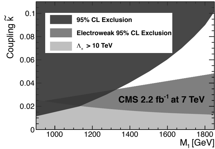
Figure 3: The 95% CL exclusion region for the RS1 graviton model in the M_1-\tilde{k} plane. The expected limits coincide very closely with the measured limits and so are not shown in the figure. Also shown are bounds due to electroweak constraints [27] and naturalness ( \Lambda_\pi > 10 TeV). Perturbativity requirements bound \tilde{k} \lesssim 0.10 .
