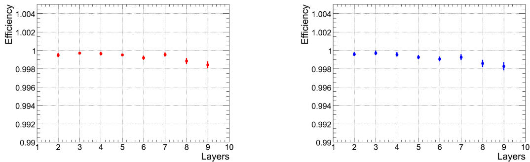
Figure 24: Summary of layer efficiency at room temperature (left) and at T = -10^\circ\text{C} (right).
