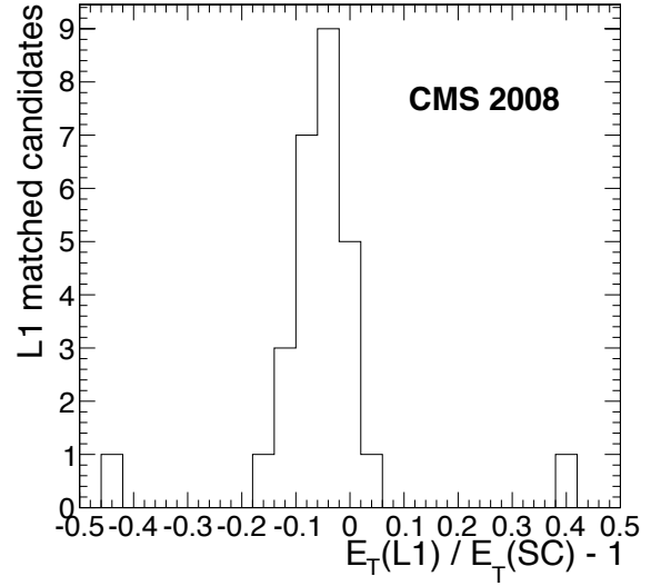
Figure 21: Level-1 e/\gamma E_T resolution for E_T(\text{L1}) > 10 GeV. The non-zero mean results from a combination of factors and is compatible with the LSB of E_T(\text{L1}) .
