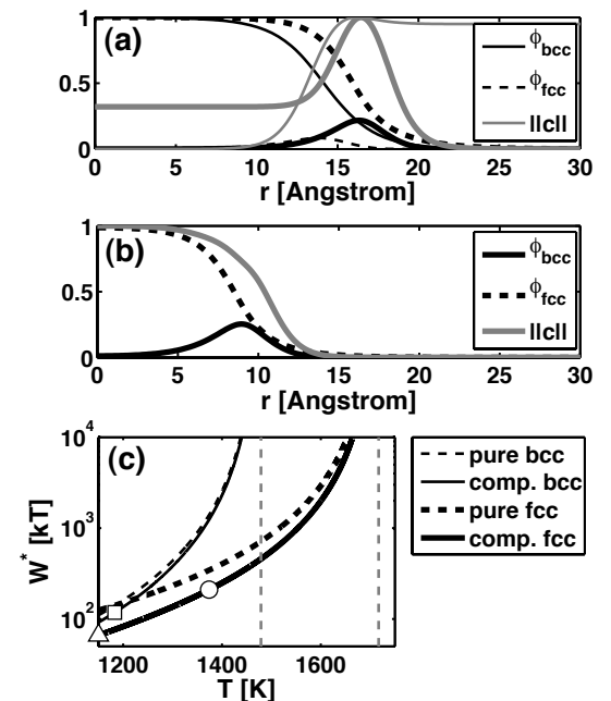
FIG. 3: Crystal nuclei in \text{Fe}_{50}\text{Ni}_{50} : Notations are as for Fig. 2. The respective temperatures are T = 1373.5 K and 1183 K for panel (a) and 1150 K for panel (b). Note that ||c|| \in [0, 1] .
