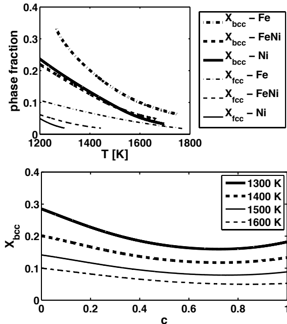
FIG. 5: Volume fraction of the third phase ("surface phase") in composite nuclei: (a) Temperature dependence of bcc fraction in composite-fcc nuclei (heavy lines), and of fcc fraction in composite-bcc nuclei (thin lines). (b) bcc fraction vs. Ni concentration at different temperatures.
