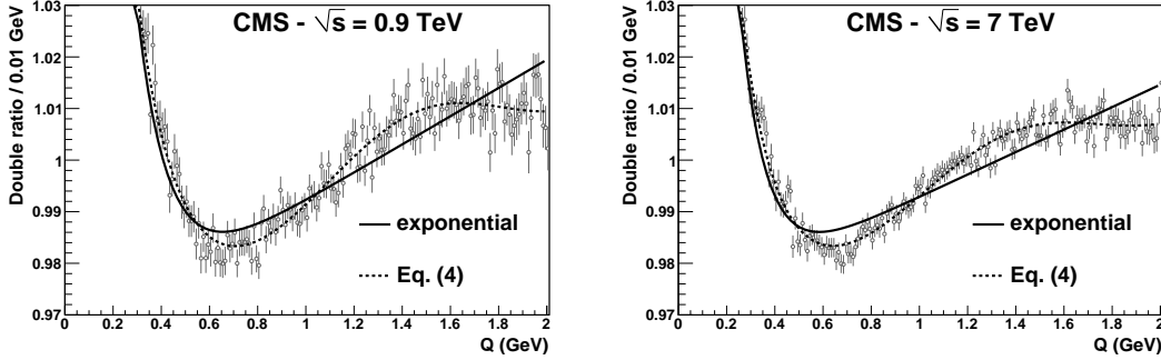
Figure 5: Detail of the distribution of the double ratio \mathcal{R} for \sqrt{s} = 0.9 (left) and 7 TeV (right). The dotted lines correspond to fits with Eq. (4), and the solid lines to exponential fits. Note the enlarged scale on the y axis. The error bars are statistical only.
