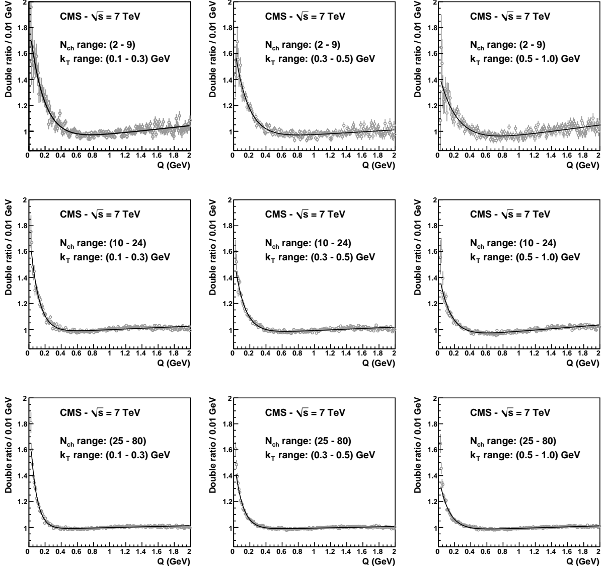
Figure 2: Distributions of the double ratio \mathcal{R} as a function of Q , for three intervals in k_{\text{T}} and three intervals in charged-particle multiplicity in the event, N_{\text{ch}} , for \sqrt{s} = 7 TeV. The lines are the results of fits using the exponential parametrization for \Omega(Qr) , with the values of the parameters given in Table 3. The error bars are statistical only.
