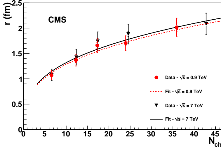
Figure 4: Parameter r as a function of the charged-particle multiplicity in the event, N_{\text{ch}} , for \sqrt{s} = 0.9 and 7 TeV. The dotted and solid lines represent the results of the fits described in the text to the 0.9 and 7 TeV data, respectively. The inner error bars represent the statistical uncertainties and the outer error bars the statistical and systematic uncertainties, added in quadrature. The systematic uncertainties are dominating and are point-to-point correlated.
