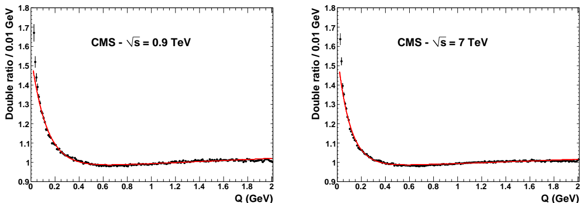
Figure 1: Distribution, for Q > 0.02 GeV, of the double ratio \mathcal{R} defined in Eq. (3), for data at \sqrt{s} = 0.9 (left) and 7 TeV (right). The reference sample is obtained from same-sign charged particles from mixed events with similar multiplicities, and the MC simulation is PYTHIA6.4 tune Z2. The lines are the results of fits using the exponential parametrization for \Omega(Qr) , with the values of the parameters given in the text. The error bars on the data points are statistical only.
