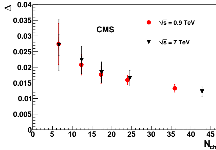
Figure 7: Depth \Delta of the dip in the anticorrelation region, as a function of the charged-particle multiplicity in the event, for \sqrt{s} = 0.9 and 7 TeV. The inner error bars represent the statistical errors and the outer error bars the statistical and systematic errors, added in quadrature. The systematic uncertainties are dominating and are point-to-point correlated.
