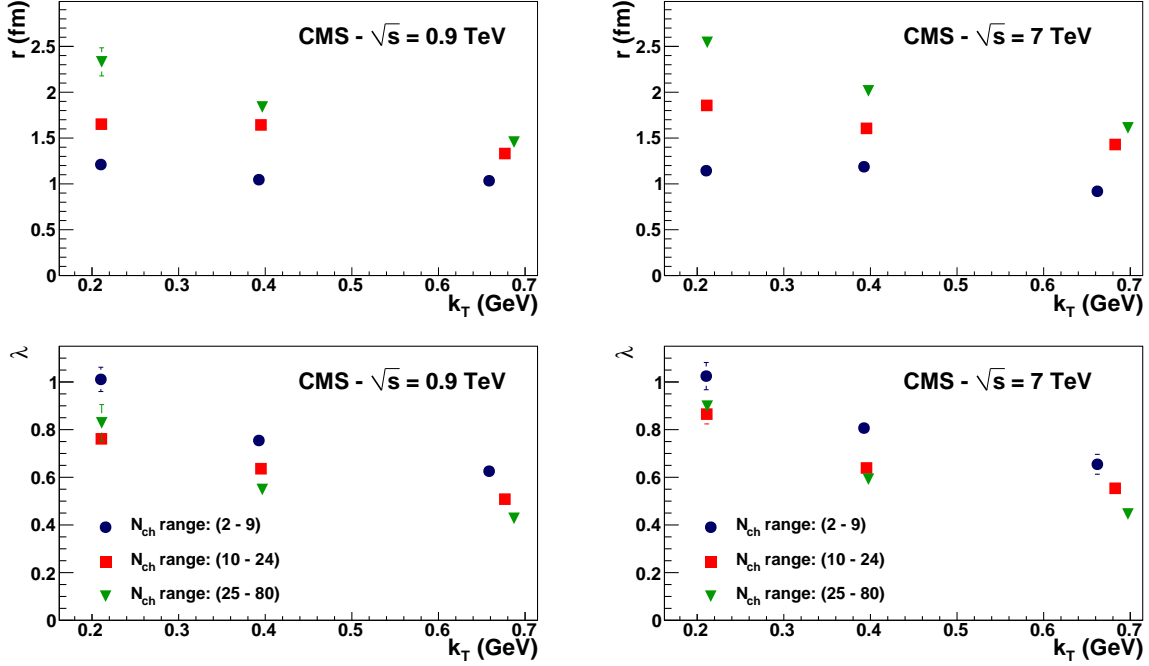
Figure 3: Values of the parameters r (top) and \lambda (bottom), as a function of k_T in three intervals of charged-particle multiplicity in the event, N_{\text{ch}} , for \sqrt{s} = 0.9 (left) and 7 TeV (right). The points are presented at the position corresponding to the mean value of k_T in the considered interval of N_{\text{ch}} . The error bars are statistical only (in some cases they are smaller than the marker size). The systematic uncertainties are discussed in the text.
