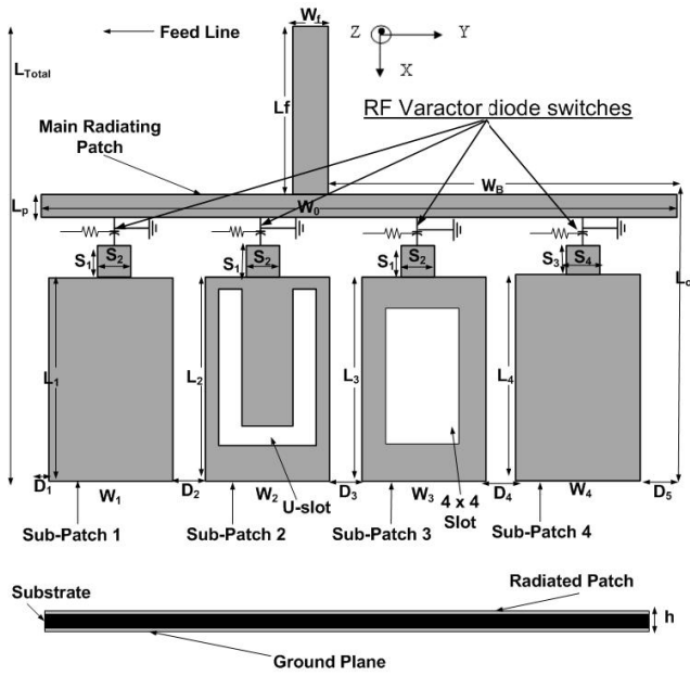
Fig. 1 The structure of the proposed antenna
