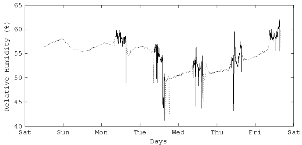
Figure 4.24: Example of relative humidity (%) in a classroom. —, Occupied hours weekday; \cdots , Unoccupied hours weekday and all hours weekend.
