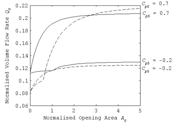
Figure 3.38: Prediction of the effect of an exposed trickle vent opening on Windcatcher ventilation rates. \theta = 0^\circ , —; \theta = 45^\circ - - -.
