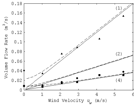
Figure 3.29: Comparison between semi-empirical predictions and the experimental measurements of Elmualim (2005b) without dampers and grill for \theta = 0^\circ . Labelled quadrants; —, prediction \Delta T = 0^\circ\text{C} ; - - -, prediction \Delta T = 10^\circ\text{C} ; \blacktriangle , quadrant 1; \blacksquare , quadrant 2; and \bullet , quadrant 4.
