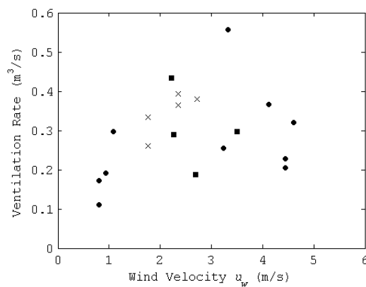
Figure 6.9: Measured ventilation rate and window area for Windcatchers with open windows. \times , ( 0.3\text{ m}^2 < A_5 < 0.5\text{ m}^2 ); \blacksquare , ( 0.5\text{ m}^2 < A_5 < 1\text{ m}^2 ); \bullet , ( 1.5\text{ m}^2 < A_5 < 2\text{ m}^2 ).
