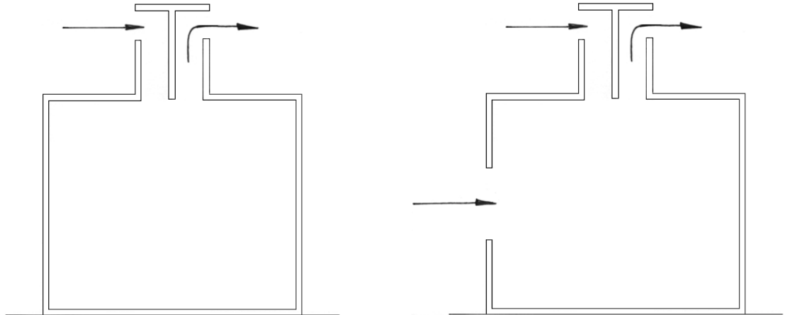
Figure 2.7: Top down ventilation, wind-catcher. Figure 2.8: Top down ventilation, wind-catcher with façade opening.
