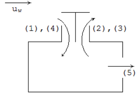
Figure 3.15: Secondary flow paths for a room ventilated by a Windcatcher with wind incident at \theta = 0^\circ , and a façade opening with C_{p5} < 0 . Labelled quadrants.
