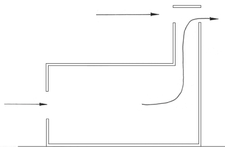
Figure 2.5: Stack ventilation.
