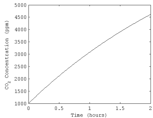
Figure 7.4: Predicted CO 2 concentration in a classroom with background ventilation.
