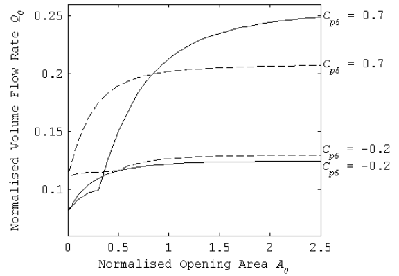
Figure 3.36: Prediction of the effect of the area of an exposed façade opening on Windcatcher ventilation rates. \theta = 0^\circ , - - -; \theta = 45^\circ —.
