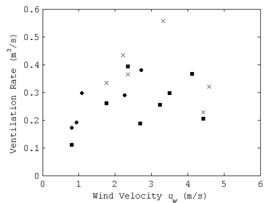
Figure 6.10: Measured ventilation rate and window location for Windcatchers with open windows. \times , front ( \theta = 0^\circ ); \blacksquare , side ( \theta = 90^\circ or \theta = 270^\circ ); \bullet , rear ( \theta = 180^\circ ).
