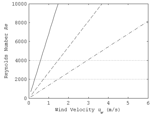
Figure 3.21: Predicted Reynolds Number in Windcatcher quadrants. Quadrant 1, —; quadrant 2, ---; quadrant 4, - · - ·.
