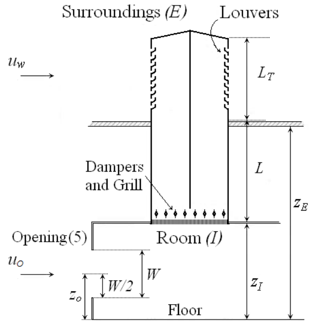
Figure 3.2: Side view of Windcatcher.
