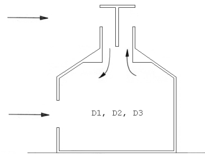
Figure 4.15: Ventilation strategy, school D.
