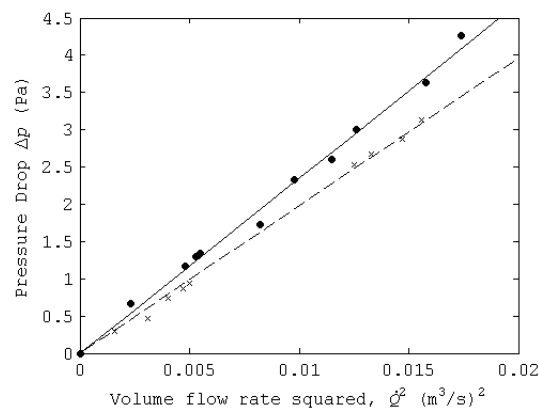
Figure 3.26: Measurements by Parker & Teekeram (2004b) of flow rate into and out of the top section of a Windcatcher. Air flow out through quadrant, ● and —; Air flow in through quadrant, × and - - -.
