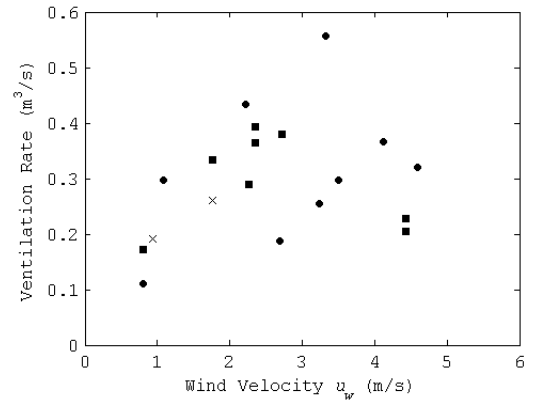
Figure 6.8: Measured ventilation rate and \Delta T for Windcatchers with open windows. \times , ( -5^\circ\text{C} < \Delta T < 0^\circ\text{C} ); \blacksquare , ( 0^\circ\text{C} < \Delta T < 5^\circ\text{C} ); \bullet , ( 5^\circ\text{C} < \Delta T < 15^\circ\text{C} ).
