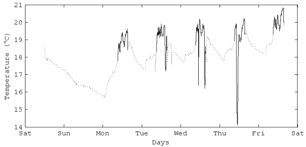
Figure 4.23: Example of air temperature in a classroom ( ^{\circ}\text{C} ). —, Occupied hours weekday; \cdots , Unoccupied hours weekday and all hours weekend.
