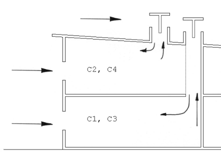
Figure 4.14: Ventilation strategy, school C.
