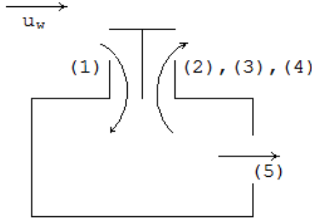
Figure 3.14: Primary flow paths for a room ventilated by a Windcatcher with wind incident at \theta = 0^\circ , and a façade opening with C_{p5} < 0 . Labelled quadrants.
