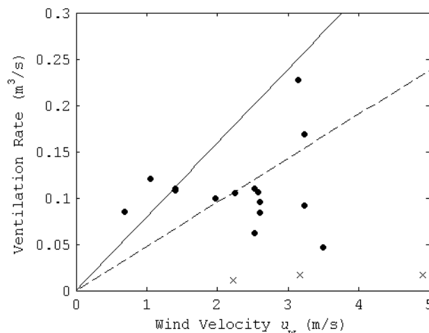
Figure 6.2: Ventilation rates for an autonomous 800 mm square Windcatcher. —, prediction \theta = 0^\circ ; ---, prediction \theta = 45^\circ ; •, measurement L \leq 1\text{ m} ; ×, measurement L > 1\text{ m} .
