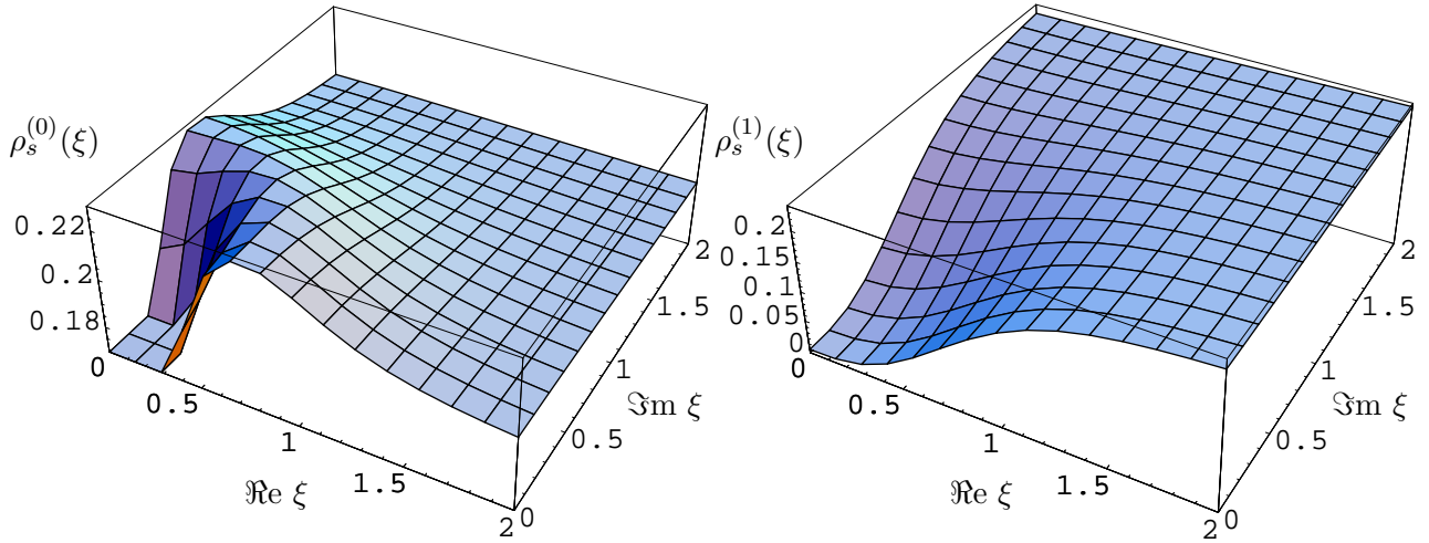
Figure 3: The microscopic density at \tau = 0.5 for a = 0 (left) and a = 1 (right) massless flavors.
