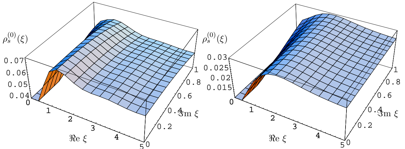
Figure 2: The quenched microscopic density ( a = 0 ) at \alpha^2 = 1.6 (left) and \alpha = 2.5 (right).
