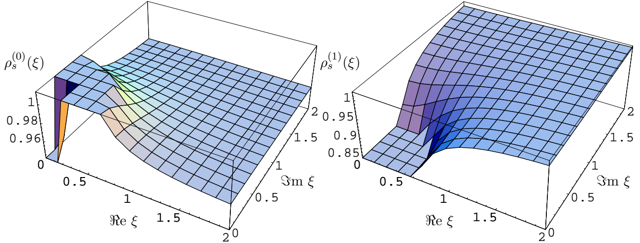
Figure 4: The microscopic density at \tau \approx 0.9 for a = 0 (left) and a = 1 (right) massless flavors.
