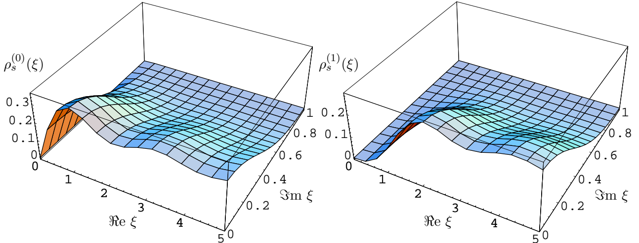
Figure 1: The microscopic density at \alpha^2 = 0.6 for a = 0 (left) and a = 1 (right) massless flavors.
