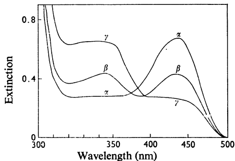
Fig. 2. Spectra of the subforms of aspartate aminotransferase
