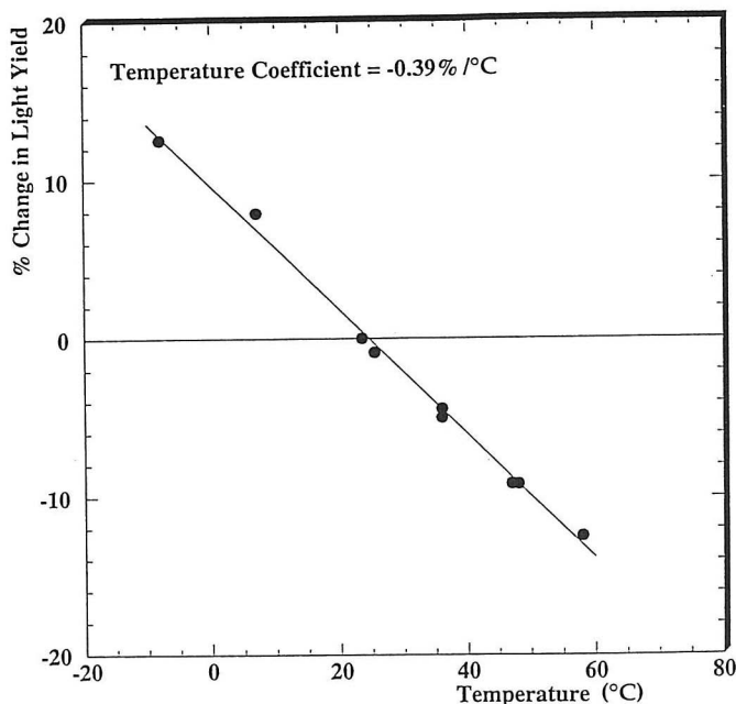
Figure 2 The measured variation of light yield with temperature for a fluorohafnate glass doped with \text{CeF}_3 .
