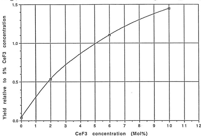
Figure 1 The measured light yield plotted against \text{CeF}_3 concentration, for a set of glasses of composition 'HBCeAN'. The yield has been normalised to unity for 5% \text{CeF}_3 concentration.
