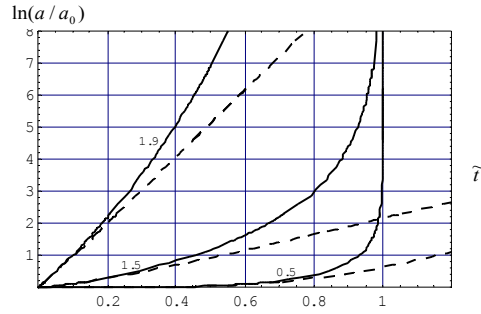
Figure1. Creep crack length vs. time for different b (local approach)
