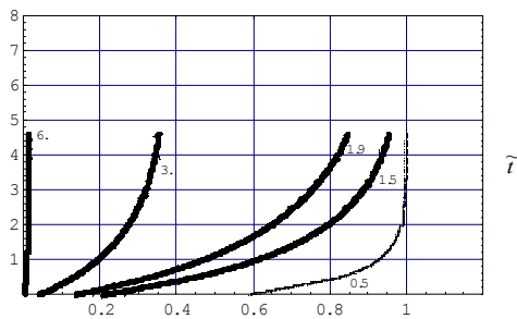
Figure 3. Creep crack length vs. time for different b (non-local approach)
