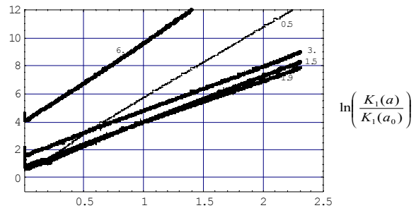
Figure 4. Creep crack growth rate vs. stress intensity factor for different b (non-local approach).
