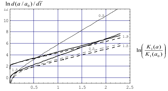
Figure 2. Creep crack growth rate vs. stress intensity factor for different b (local approach).
