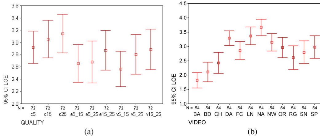
Fig. 9. Mean and 95% significance plot for QoP-LoE, dependent on (a) quality and (b) video type.
