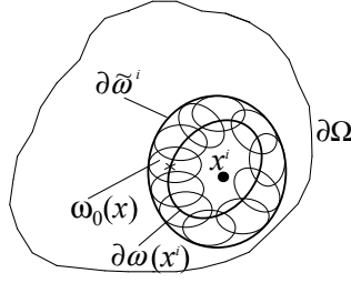
Figure 5: A localization domain \omega(x^i) and a total localization domain \tilde{\omega}^i associated with a collocation point x^i of a body \Omega for a mesh-less discretization
