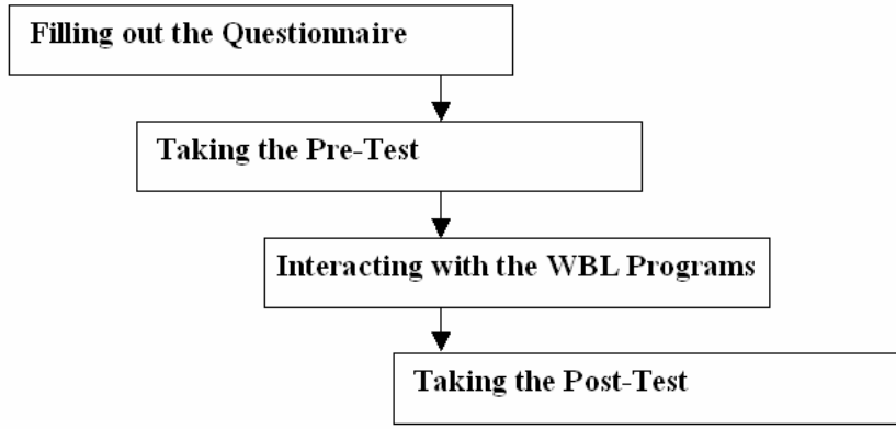
Figure 3: Procedures
