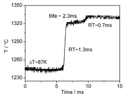
Fig. 1 Temperature time plot of a high-speed photo diode from a parabolic flight experiment with a Fe 90 Ni 10 droplet undercooled 87 K showing the double-recalescence with intermediate metastable phase (RT = recalescence time).
