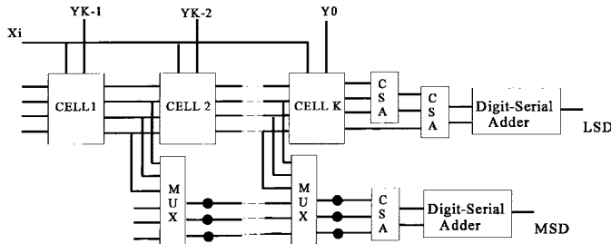
Fig. 12. Twin-pipe digit-serial multiplier.
