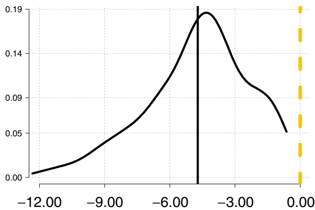
Fig. 7 Kernel estimated density of skewness. The vertical dashed-dotted line is 0. The solid vertical line is the mean
