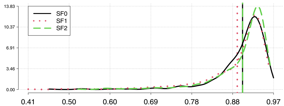
Fig. 5 Kernel estimated densities of efficiencies. Vertical lines are respective means
