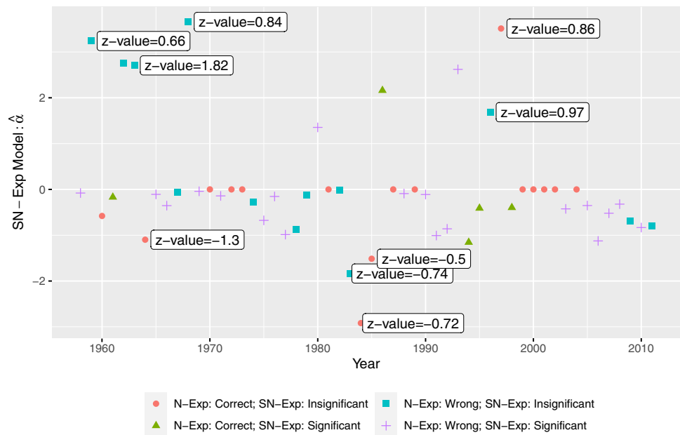
Fig. 9 The estimated skewness coefficient by year
