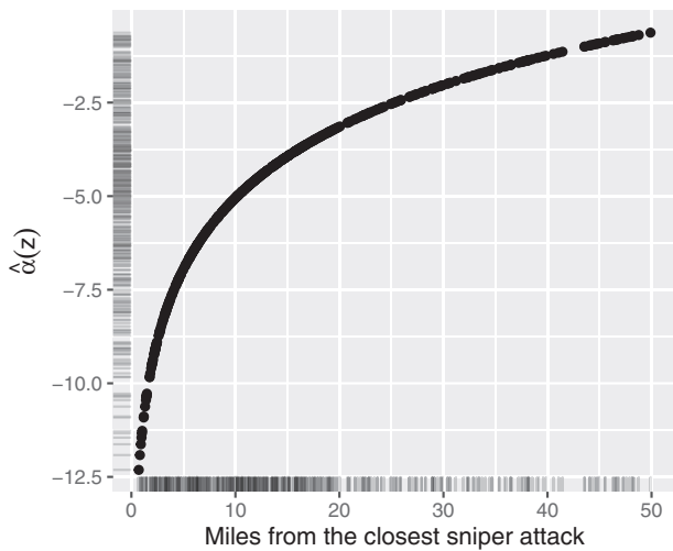
Fig. 6 The estimate of skewness (fitted values) plotted against the respective determinant. The rug plot on each axis essentially shows a one-dimensional heatmap
