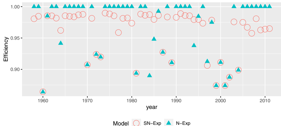
Fig. 10 The average of the efficiency score estimated by N-Exp and SN-Exp models by year
