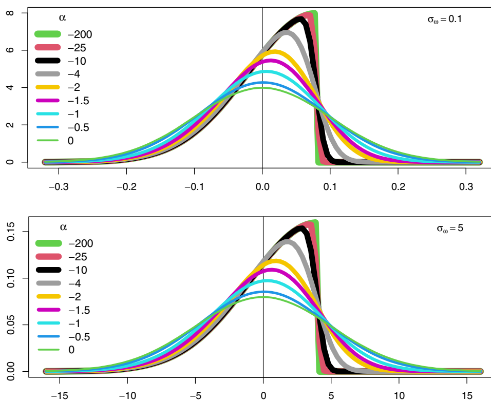
Fig. 1 pdf of the skew-normal random variable
