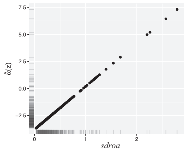
Fig. 4 The estimate of skewness (fitted values) plotted against the determinant (Model SF2). The rug plot on each axis essentially shows a one-dimensional heatmap
