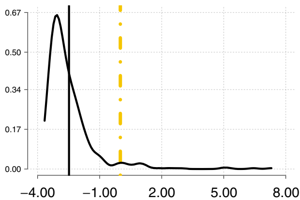
Fig. 3 Kernel estimated densities of skewness (Model SF2). The vertical dash-dotted line is 0. The solid vertical line is the mean
