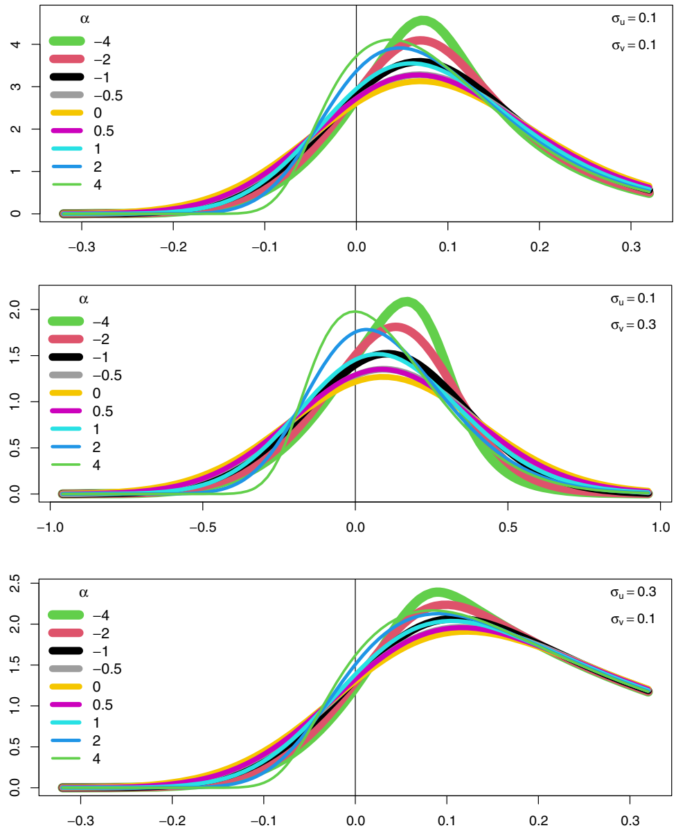
Fig. 2 pdf of the convolution of skew-normal and exponential random variables, \epsilon = v - pu , where p = -1
