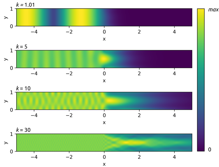
Figure 10. The magnitude of the potential field ( |\psi_1| for x < 0 and |\psi_2| for x > 0 ) at the first EP3 (absorbing walls) of Tab. 1, computed for different frequency values. The colour scale ranges from 0 to the max of each field. Note the focal spot occurring for k \geq 5 .
