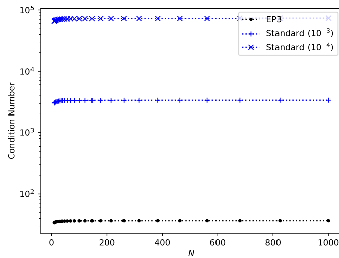
Figure 7. The condition number of the linear system (logarithmic scale) against the number of modes N . The black curve is the enhanced matching scheme with the additional wave functions, the blue ones are the standard matching scheme where both wall admittances have been shifted a distance of \delta = 10^{-3} or \delta = 10^{-4} respectively from the EP value.
