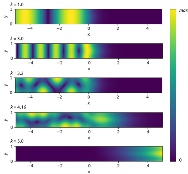
Figure 13. The magnitude of the potential field ( |\psi_1| for x < 0 and |\psi_2| for x > 0 ) at EP3-PT (one passive and one active wall), computed at different frequency values. The colour scale ranges from 0 to the max of each field.
