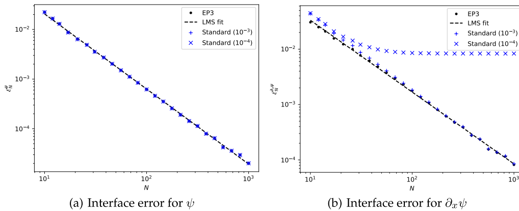
Figure 6. The error at the interface (logarithmic scale) against the number of modes N of the truncated series. The markers are data and the dashed line is the least mean square fit with the ansatz \mathcal{E}(N) = C/N^p . The black points are the exact matching scheme with additional wave functions, the blue markers are the standard matching scheme where both admittance values have been shifted a distance of \delta = 10^{-3} or \delta = 10^{-4} respectively from the EP value.
