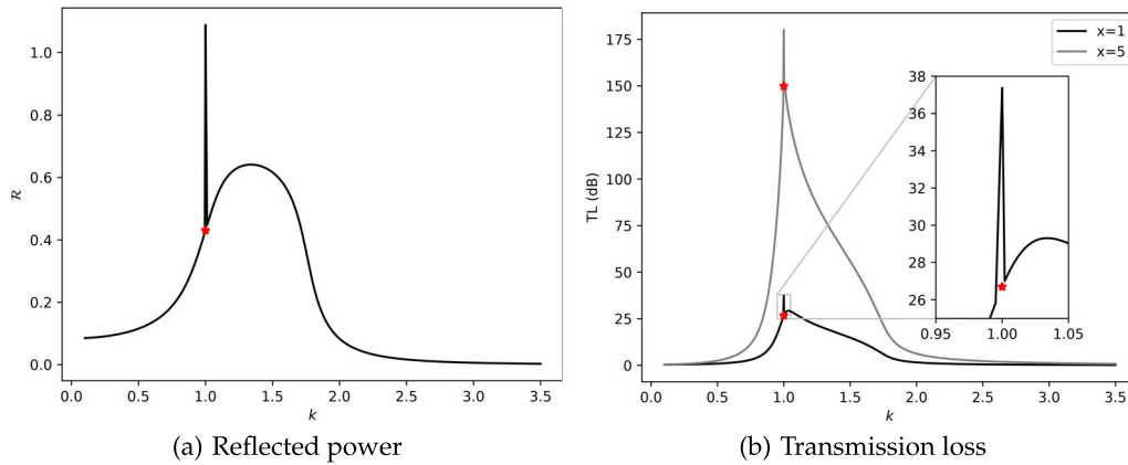
Figure 3. The (a) reflected power and (b) transmission loss at x = 1 and x = 5 for a SDOF liner. The spikes are erroneous, the stars indicate the correct values obtained using the enhanced matching scheme at the EP3.
