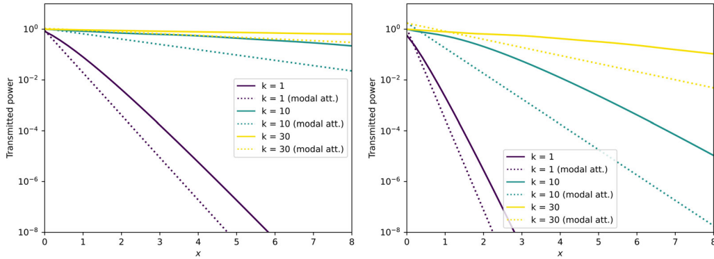
Figure 8. The transmitted power (logarithmic scale) against x for k = 1, 10, 30 : (a) at the first Tester EP2, (b) at the first EP3 with absorbing walls. Solid lines correspond to the numerical solution, computed with N = 60 modes, and dotted lines show power associated with the usual separable s_1 mode, i.e. \mathcal{P}'_2(x) .
