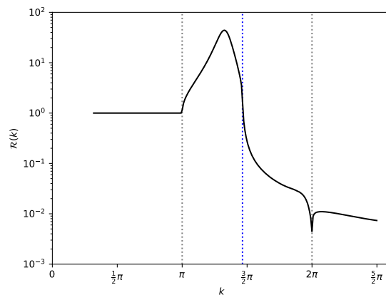
Figure 12. Reflected power (logarithmic scale) at EP3-PT (one passive and one active wall) against frequency k .
