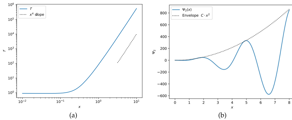
Figure 11. (a) Evolution of the transmitted power along the waveguide (logarithmic scales), (b) the magnitude (envelope) and real part of the potential \psi_2(x, 0.5) at k = 5 for the EP3-PT (one passive and one active wall) parameters.
