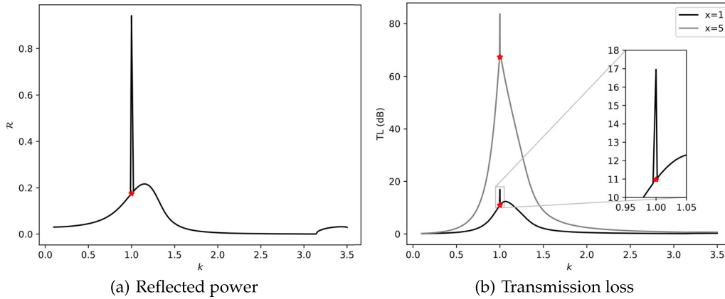
Figure 4. The (a) reflected power and (b) transmission loss at x = 1 and x = 5 for a SDOF liner. The spikes are erroneous, the stars indicate the correct values obtained using the enhanced matching scheme at Tester's EP2.
