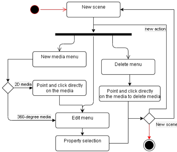
FIGURE 5. AMUSEVR - Activity diagram.
