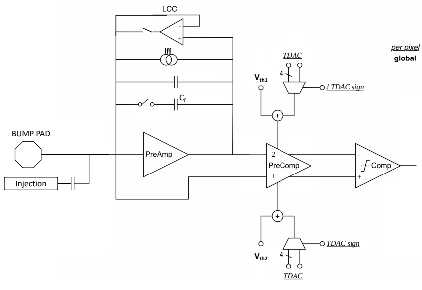
Figure 8. Schematic of the Differential front-end implemented in the RD53A chip [13].
