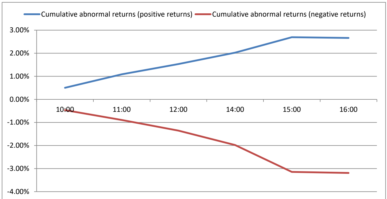
Figure L.3: Dynamics of cumulative abnormal returns: case of SSE COMPOSITE
