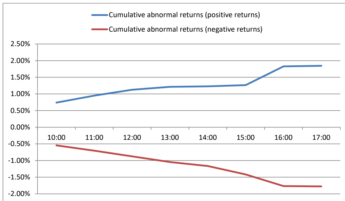
Figure C.3: Dynamics of cumulative abnormal returns, SP500
