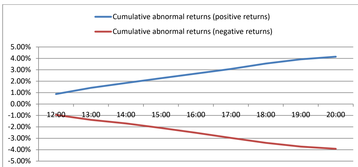
Figure E.3: Dynamics of cumulative abnormal returns: case of FTSE 100
