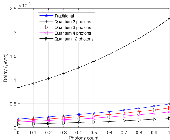
FIGURE 3. Latency of the networks, quantum and traditional showing the effect of delay gain when using different number of photons.
