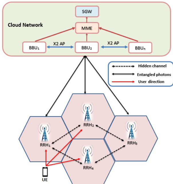
FIGURE 1. Quantum handover process architecture.
