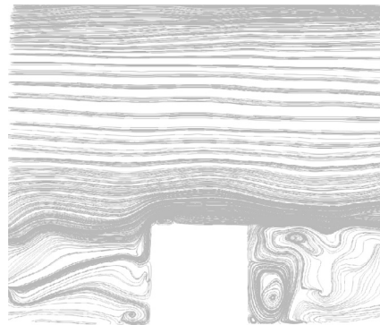
Fig. 11. LES instantaneous streamlines x-y plane, z/H=2 .
