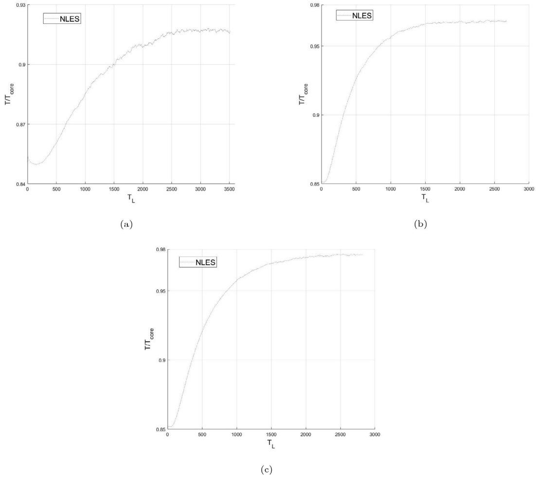
Fig. 4. Temperature development of different points in the epoxy layer as shown in Fig. 3 and Table 1.
