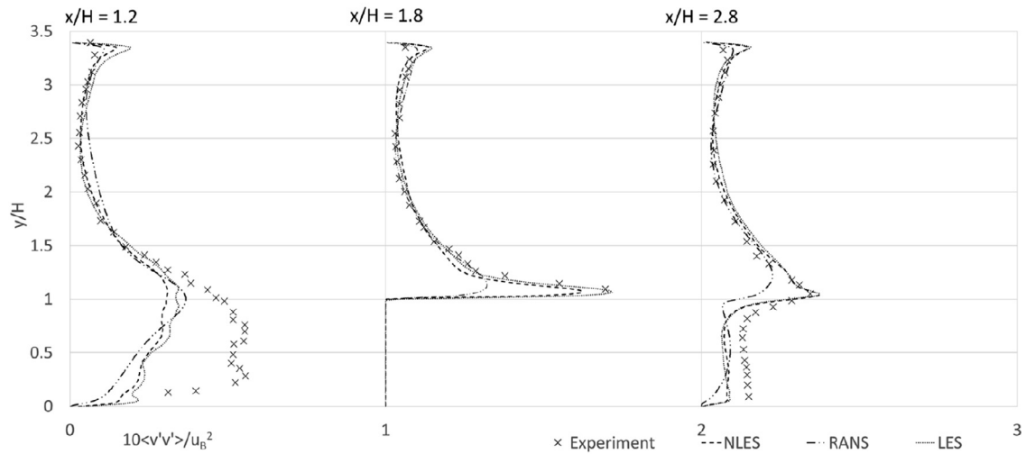
(b) Normalised resolved \langle v'v' \rangle stress
