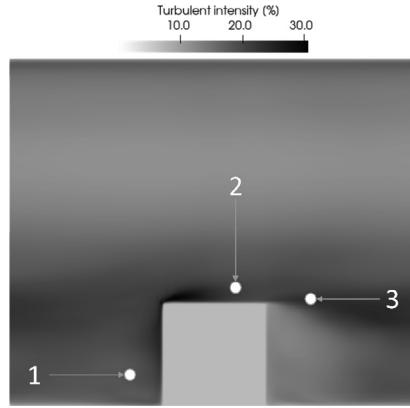
Fig. 10. Turbulent intensity with indications of positions of energy spectra's.
