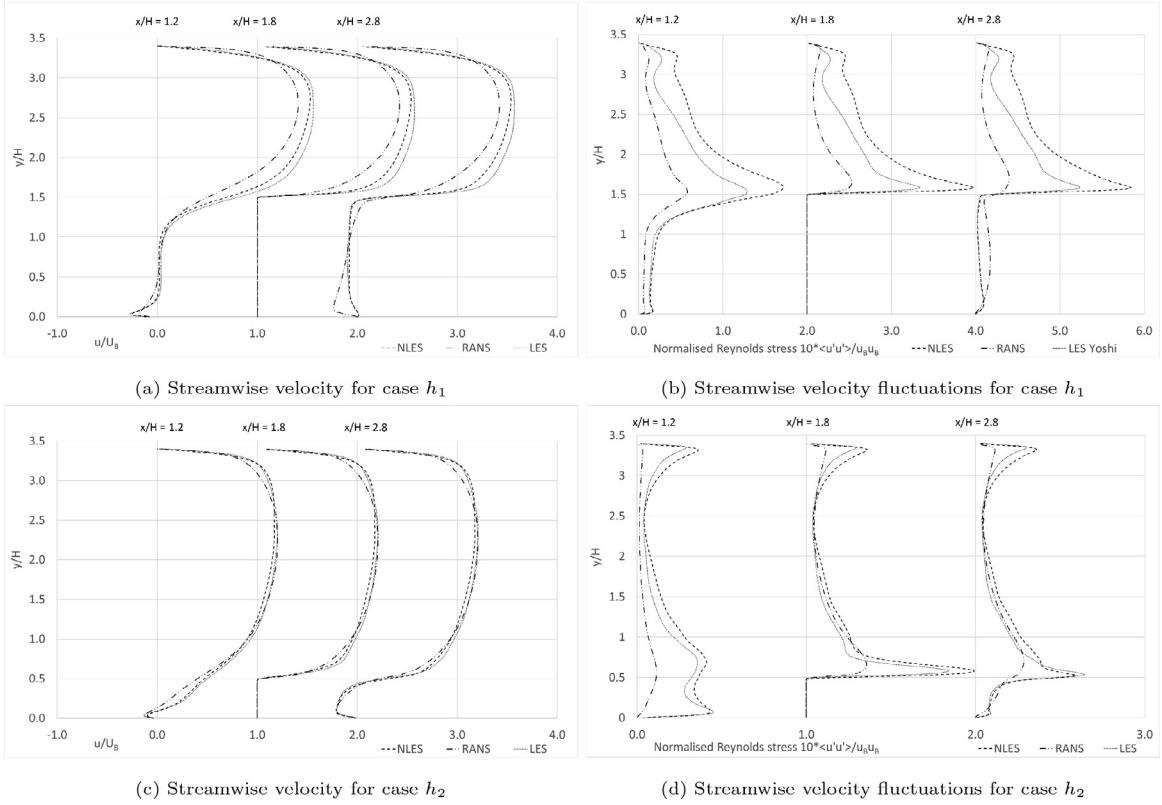
Fig. 20. Time averaged streamwise velocity and velocity fluctuations for three positions.
