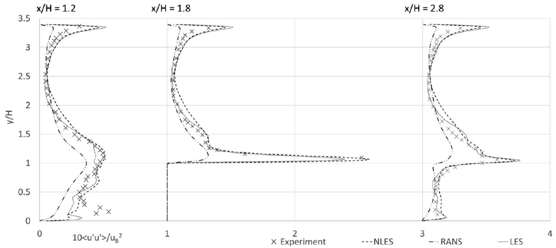
(a) Normalised resolved \langle u'u' \rangle stress
