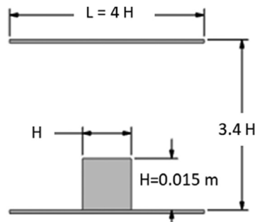
Fig. 1. Sketch of flow domain.
