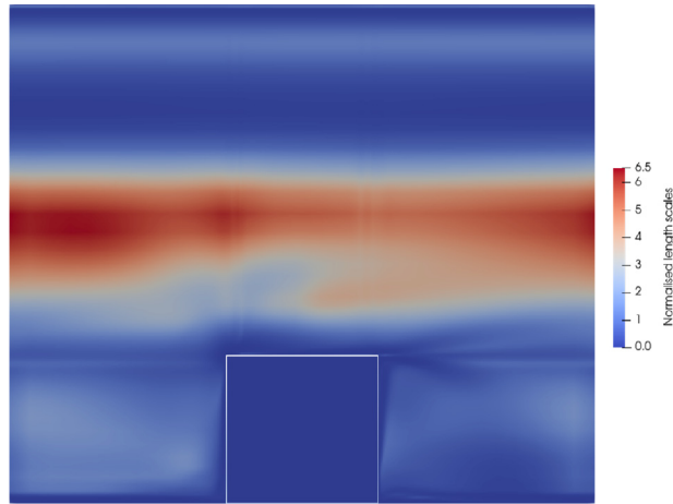
Fig. 13. Normalised length scales RANS, z/H=2 .
