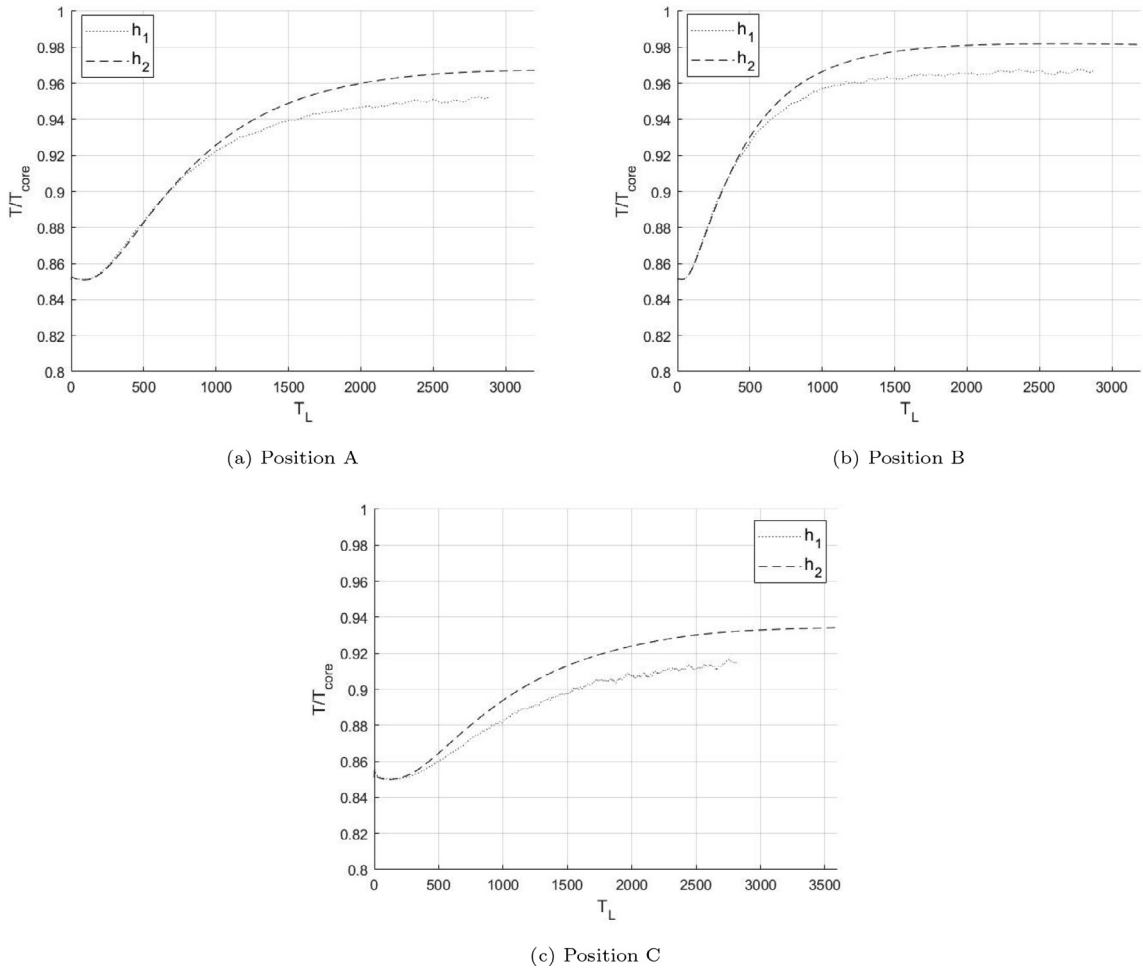
Fig. 19. Temperature NLES development of points in epoxy layer.
