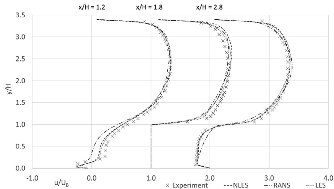
Fig. 8. Streamwise velocity comparison.
