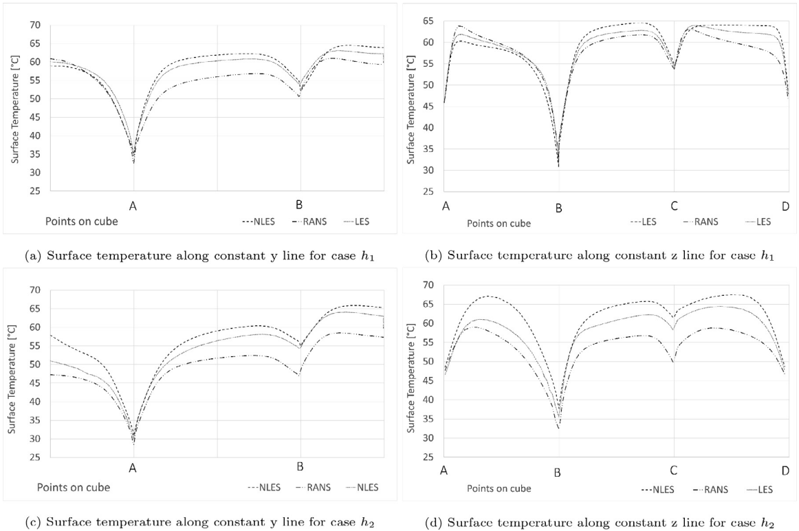
Fig. 21. Surface temperature plots for the two cases.
