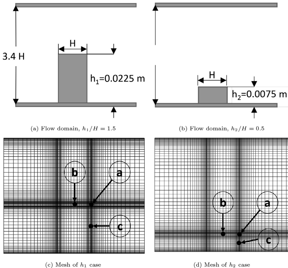
Fig. 18. Flow domains and meshes for new cube heights.
