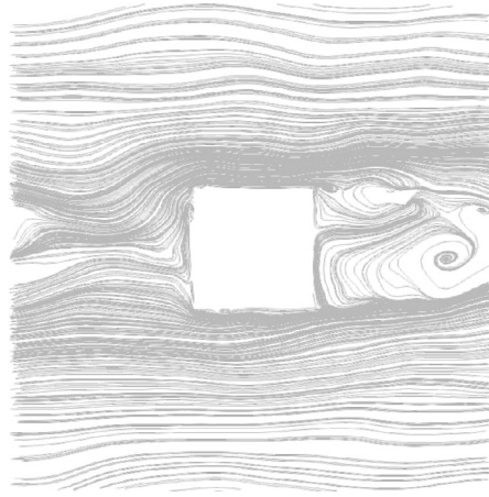
Fig. 6. LES streamlines x-z plane, y/H=0.6.
