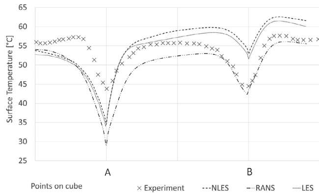
Fig. 17. Comparison of surface temperature along constant y lines.
