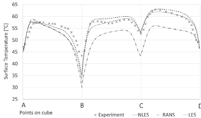
Fig. 16. Comparison of surface temperature along constant z line.
