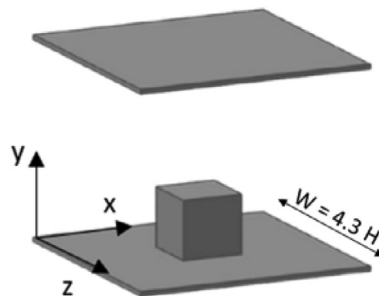
Fig. 2. 3-D view of flow domain.
