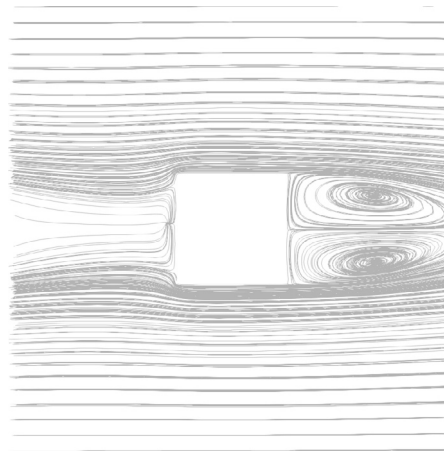
Fig. 7. RANS streamlines x-z plane, y/H=0.6.
