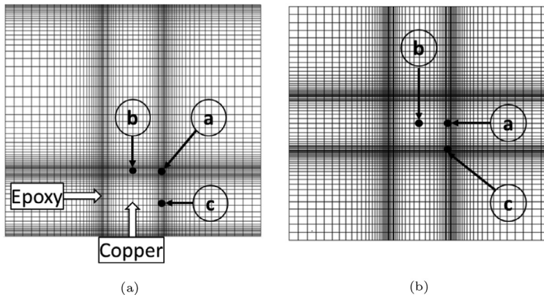
Fig. 3. Mesh in the a), x-y and b), x-z plane with indicators for conjugate temperature position.
