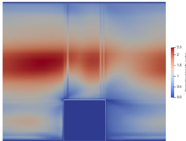
Fig. 14. Normalised length scales LES, z/H=2 .
