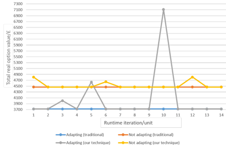
1216 Fig. 6. Comparing real option values to be enabled by adapting and retained by not adapting granularity in the scenario with single spike workload using our process against traditional analysis
