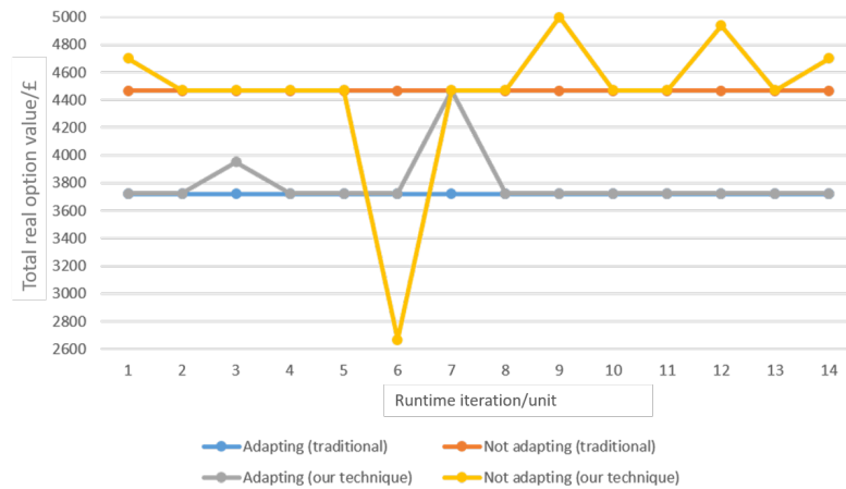
1236 Fig. 7. Comparing real option values to be enabled by adapting and retained by not adapting granularity in the scenario with multiple outliers in workload using our process against traditional analysis
