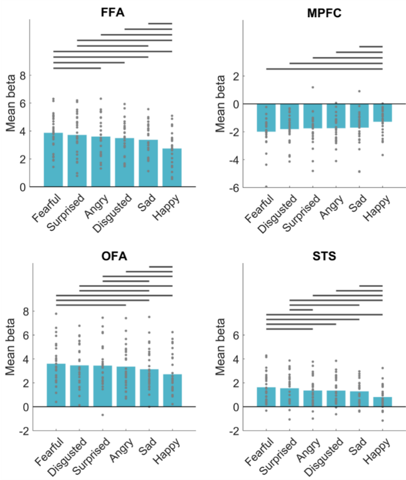
Figure 4: Univariate response to each expression category within each ROI. Horizontal black bars indicate a significant p -value for the pairwise comparison, accounting for an FDR of .05 (FFA all p < .010 ; OFA p < .022 ; STS p < .026 ; MPFC p < .013 )
