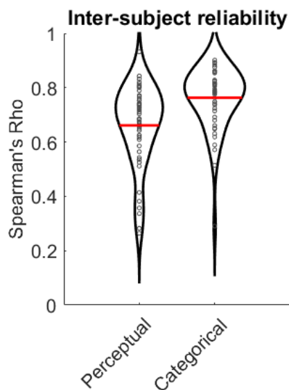
Figure S1: Inter-subject reliability. For each participant's perceptual and categorical matrices, we computed the correlation with the average of all other participants' matrices. Red bars represent the mean correlation coefficient.
