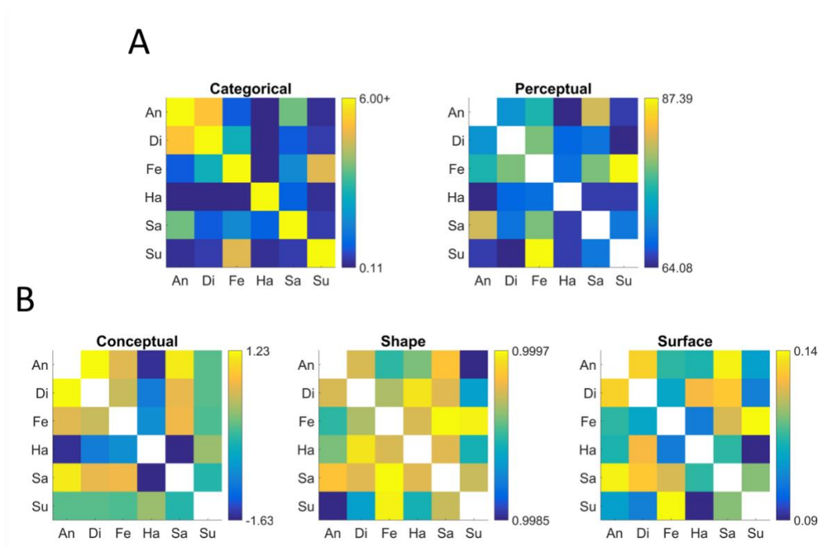
Figure 2: (A) The mean categorical matrix (left), which displays the mean number of instances pairs of emotions were confused with each other. The mean perceptual matrix (right), which displays the perceptual discrimination thresholds for each pair of expressions in the perceptual task. The colour bars are scaled to the minimum and maximum values in the off-diagonal triangles. (B) Conceptual (Fisher Z-transformed correlation coefficients; left), Shape (1-Procrustes distance; centre), and Surface (Fisher Z-transformed correlation coefficients; right) models.
