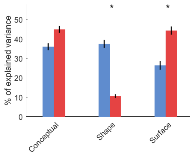
Figure S2: The mean percentages of variance explained by each of the three predictors. Blue bars show the percentage of variance explained in the Perceptual Task, red bars show the percentage of variance explained in the Categorical Task. Error bars show one standard error around the mean.
