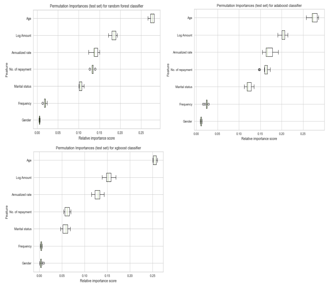
Figure 5. Feature importance for the ensemble classifiers.
