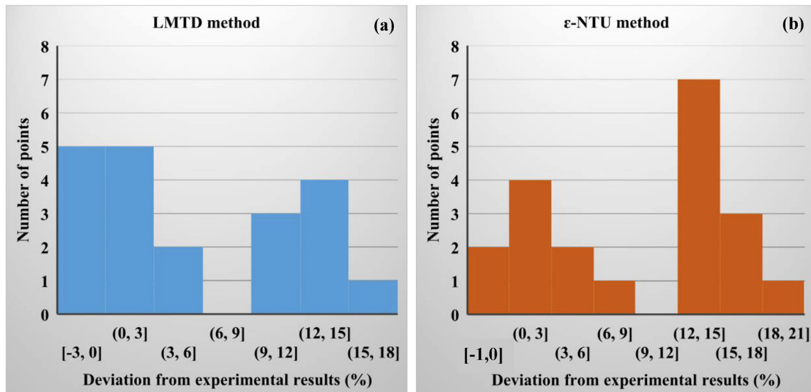
Fig. 14. Histogram of the theoretical prediction deviation from the experimental results of the HPHE effectiveness: (a) using the LMTD method, (b) using the \epsilon -NTU method.
