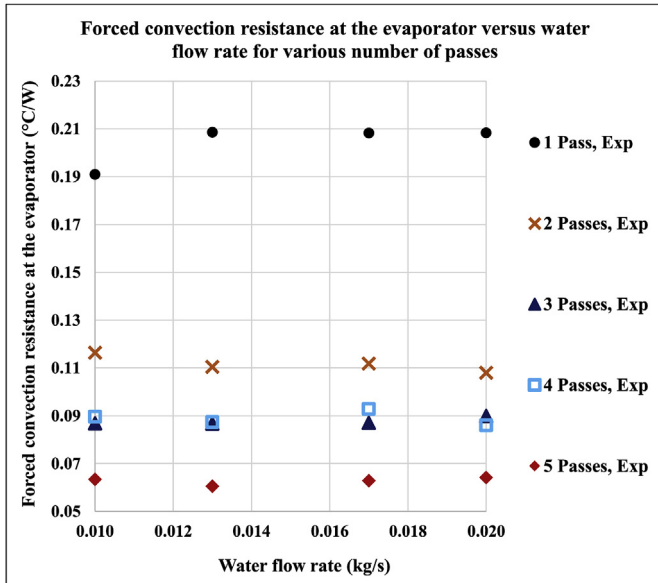
Fig. 15. Forced convection resistance at the evaporator versus water flow rate for various number of passes.
