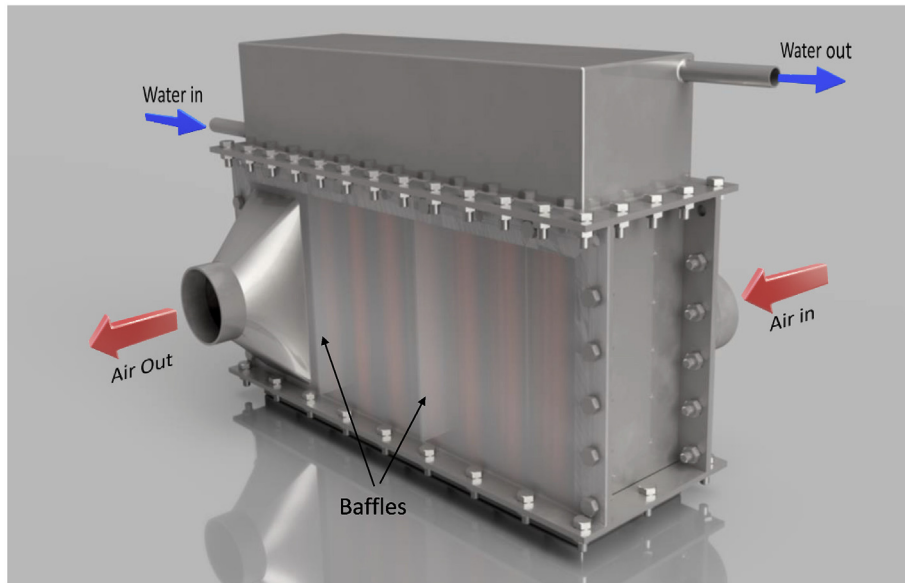
Fig. 1. Drawing of the HPHE studied.
