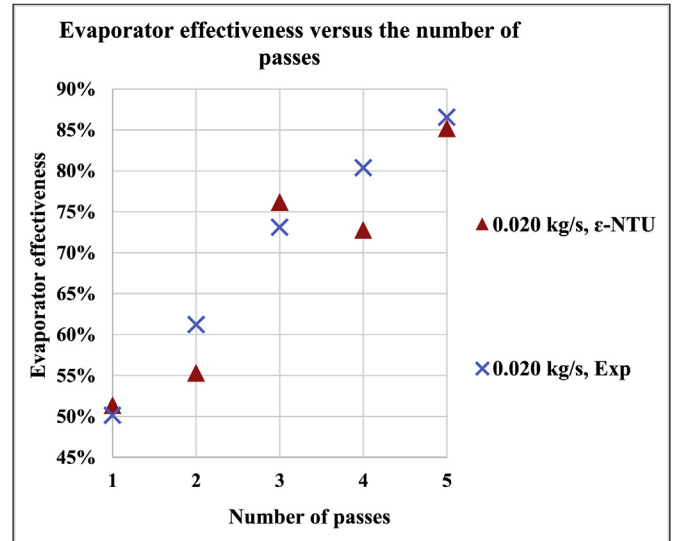
Fig. 17. Impact of the number of passes on the evaporator effectiveness.
