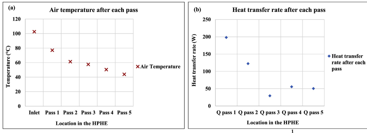
Fig. 18. Experimental results of each pass for 5 passes and water flow rate of 0.02 kg s -1 (a): Air temperature trend, (b): Heat transfer rate.
