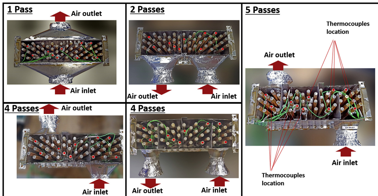
Fig. 2. Arrangement of the passes for the air at the evaporator section of the HPHE.
