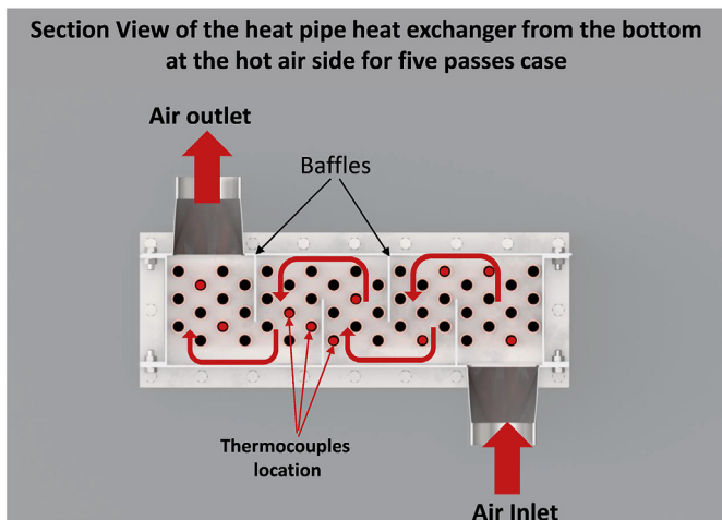
Fig. 3. Air passage through the passes of the HPHE – case of five passes.
