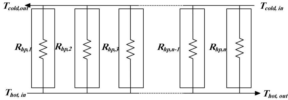
Fig. 6. Electrical-thermal resistance analogy of the HPHE.
