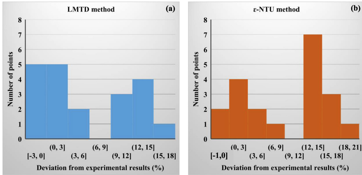
Fig. 10. Histogram of the theoretical predictions deviation from the experimental results of the heat transfer rate: (a) using the LMTD method, (b) using the ε-NTU method.
