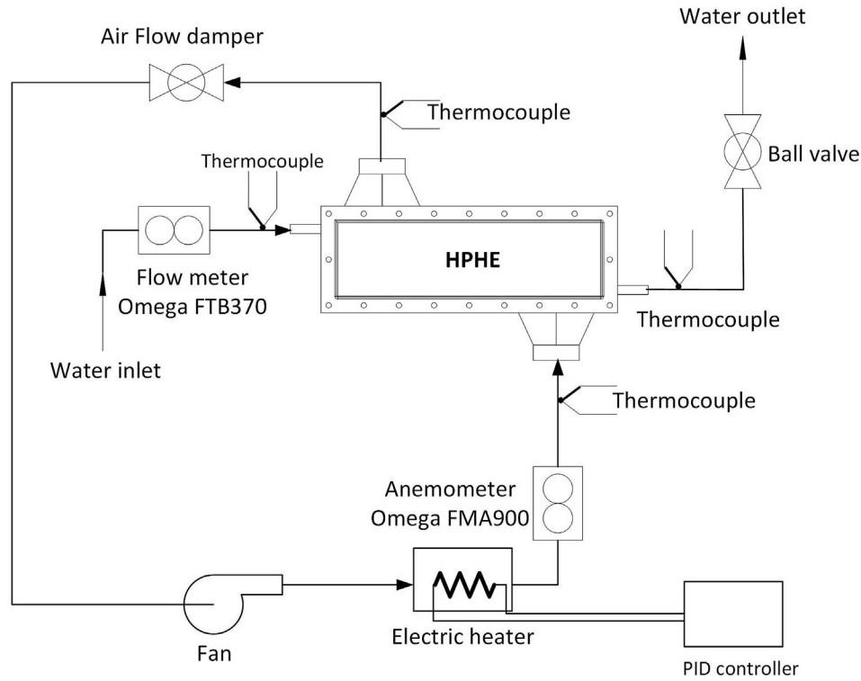
Fig. 5. Piping and Instrumentation Diagram (P&ID) of the test rig.
