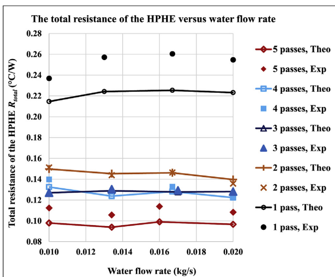
Fig. 16. The total resistance of the HPHE versus water flow rate.
