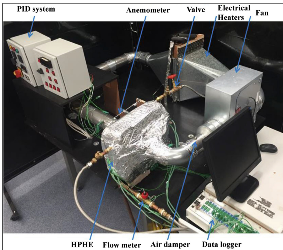
Fig. 4. Test rig of the HPHE.
