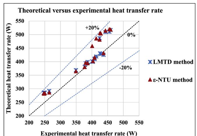
Fig. 9. A comparison between the experimental results and theoretical predictions of heat transfer rate using LMTD and \epsilon -NTU methods.
