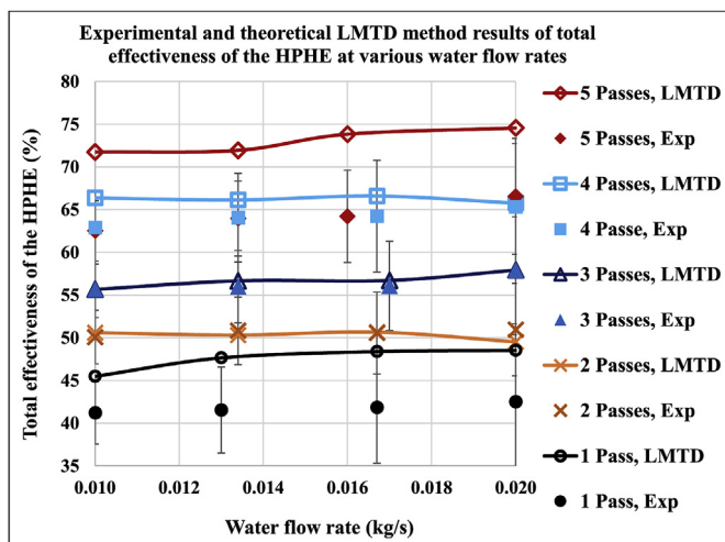
Fig. 11. Experimental and LMTD method predictions of the total effectiveness of the HPHE.
