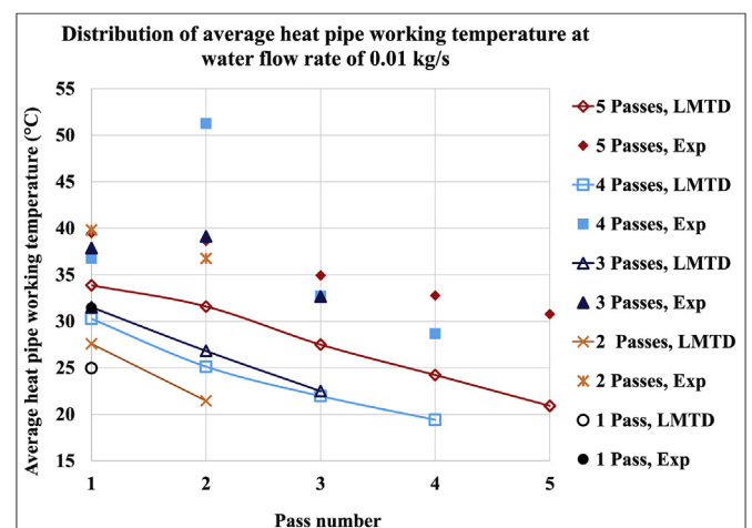
Fig. 19. Average working temperature of heat pipes and LMTD predictions for each pass at a water flow rate of 0.010 kg s -1 .
