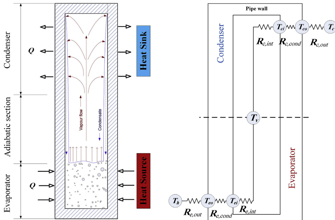
Fig. 7. Two-phase working cycle of a heat pipe and its corresponding thermal resistance model.
