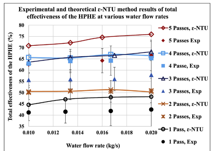
Fig. 12. Experimental and ε-NTU method predictions of the total effectiveness of the HPHE.
