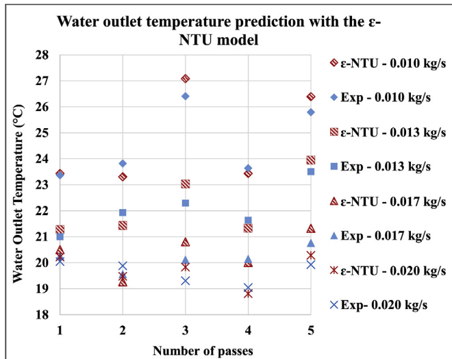
Fig. 20. Experimental water outlet temperature and LMTD predictions.
