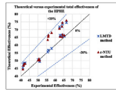
Fig. 13. A comparison between the experimental results and theoretical predictions of the HPHE total effectiveness using the LMTD and \epsilon -NTU methods.
