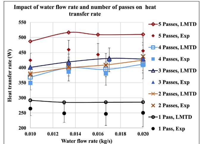
Fig. 8. Impact of water flow rate and number of passes on the total heat transfer rate.
