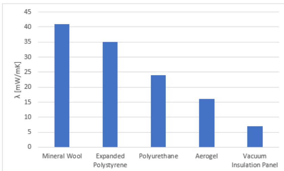
Figure 1: Thermal conductivity of five contemporary insulation materials.
