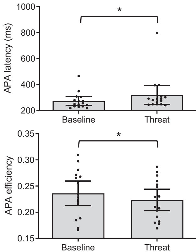
Fig. 4. Changes in APA latency (top figure) and efficiency (bottom figure) between Baseline and Threat, *p < .05 (mean \pm 95% confidence intervals, and individual data points).
