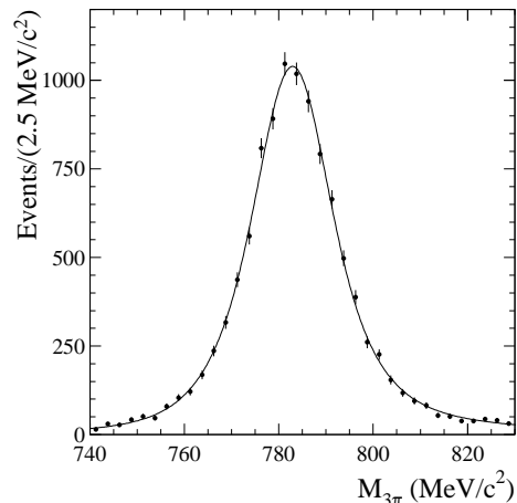
FIG. 10: The \pi^+\pi^-\pi^0 invariant mass spectrum for data events in the \omega mass region. The curve is the result of the fit described in the text.
