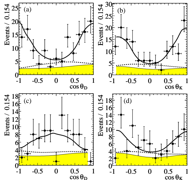
FIG. 2: Distributions of (a) \cos \theta_D and (b) \cos \theta_K for D^{*0} \rightarrow D^0 \pi^0 . Distributions of (c) \cos \theta_D and (d) \cos \theta_K for D^{*0} \rightarrow D^0 \gamma . The solid line represents the full fit model, the dashed line represents the transverse component, and the shaded region represents the combinatorial background component.
