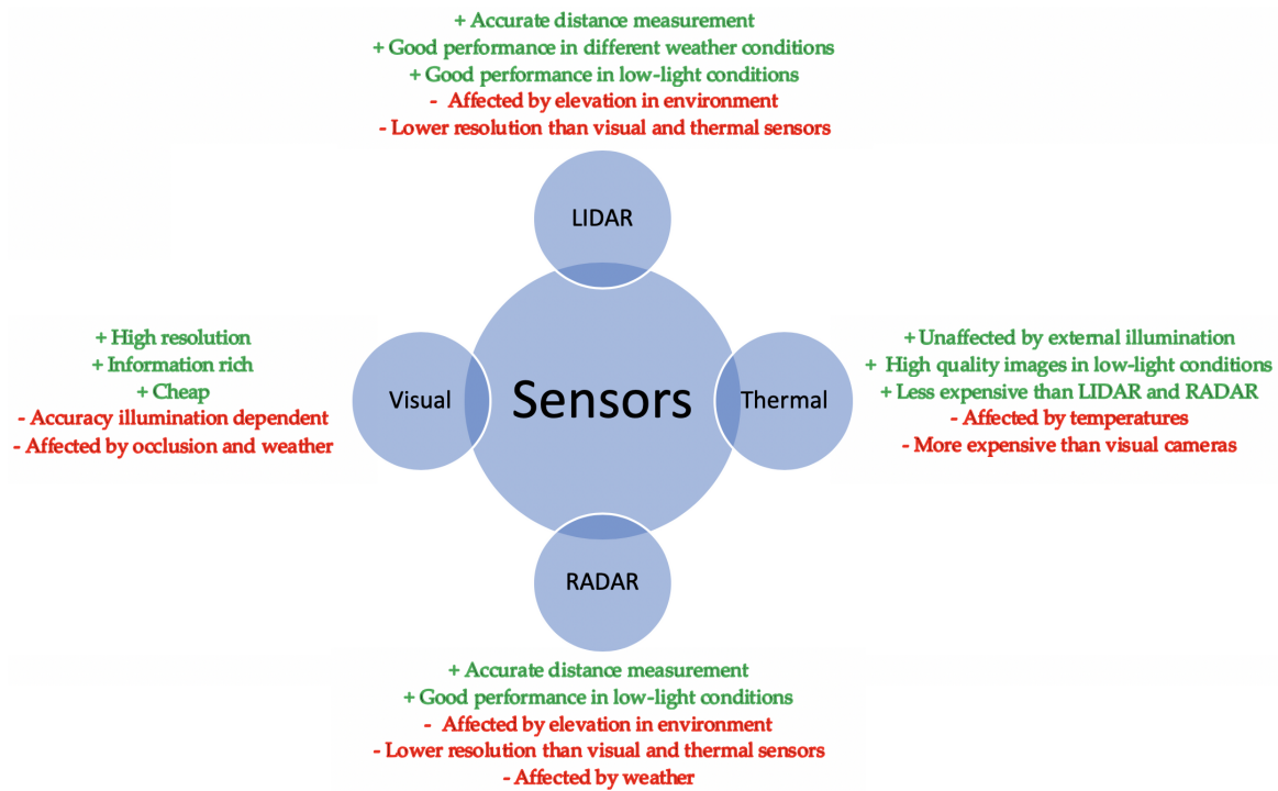
Figure 7. Sensor Comparison.
