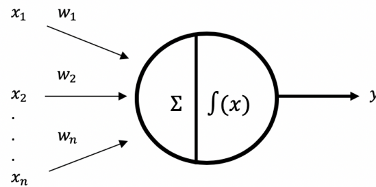
Figure 3. Single perceptron.
