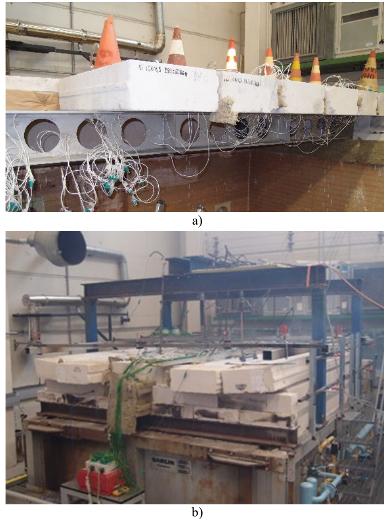
Fig. 2. a) Beam and slab construction during installation; b) Test set-up during the test.
